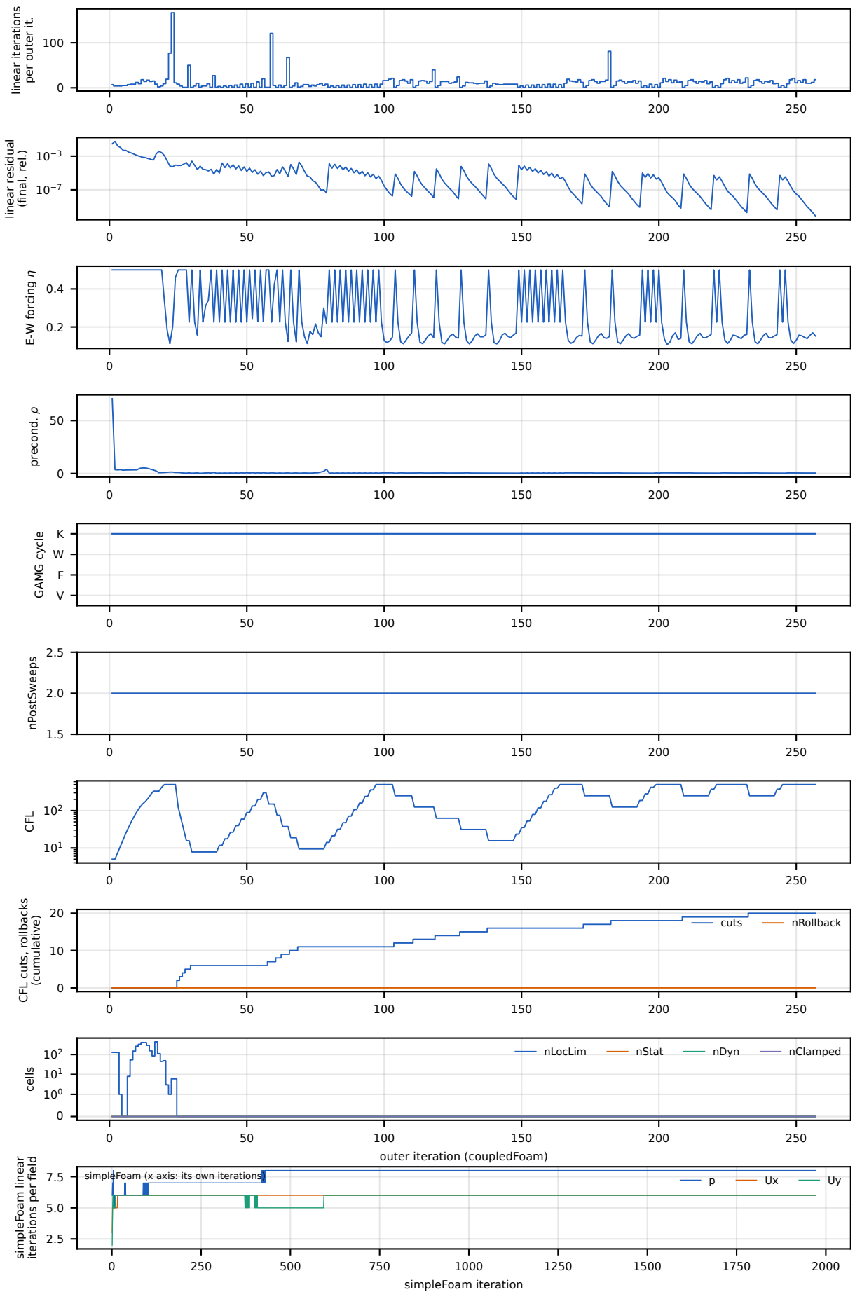
T0 cavity, Re 1000, 4 ranks: linear solver and controls per outer iteration (dotted: GAMG autoTune events)
