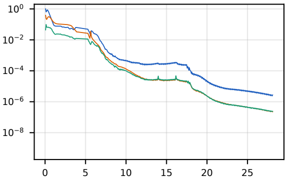
T1 pitzDaily, 1 rank: residuals (coupledFoam: combined R , momentum r_U , continuity r_p ; simpleFoam: initial residuals). Same y range; normalisations differ.
