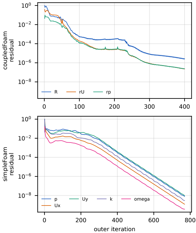
T1 pitzDaily, 1 rank: residuals (coupledFoam: combined R , momentum r_U , continuity r_p ; simpleFoam: initial residuals). Same y range; normalisations differ.
