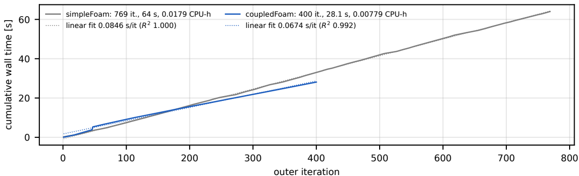
T1 pitzDaily, 1 rank: wall-clock time (dotted: linear fit; vertical dotted lines: GAMG autoTune events)
