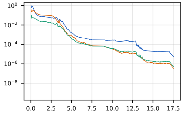
T1 pitzDaily, 4 ranks: residuals (coupledFoam: combined R , momentum r_U , continuity r_p ; simpleFoam: initial residuals). Same y range; normalisations differ.
