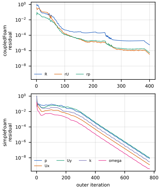
T1 pitzDaily, 4 ranks: residuals (coupledFoam: combined R , momentum r_U , continuity r_p ; simpleFoam: initial residuals). Same y range; normalisations differ.
