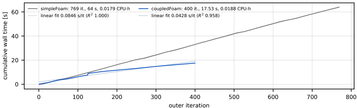
T1 pitzDaily, 4 ranks: wall-clock time (dotted: linear fit; vertical dotted lines: GAMG autoTune events)
