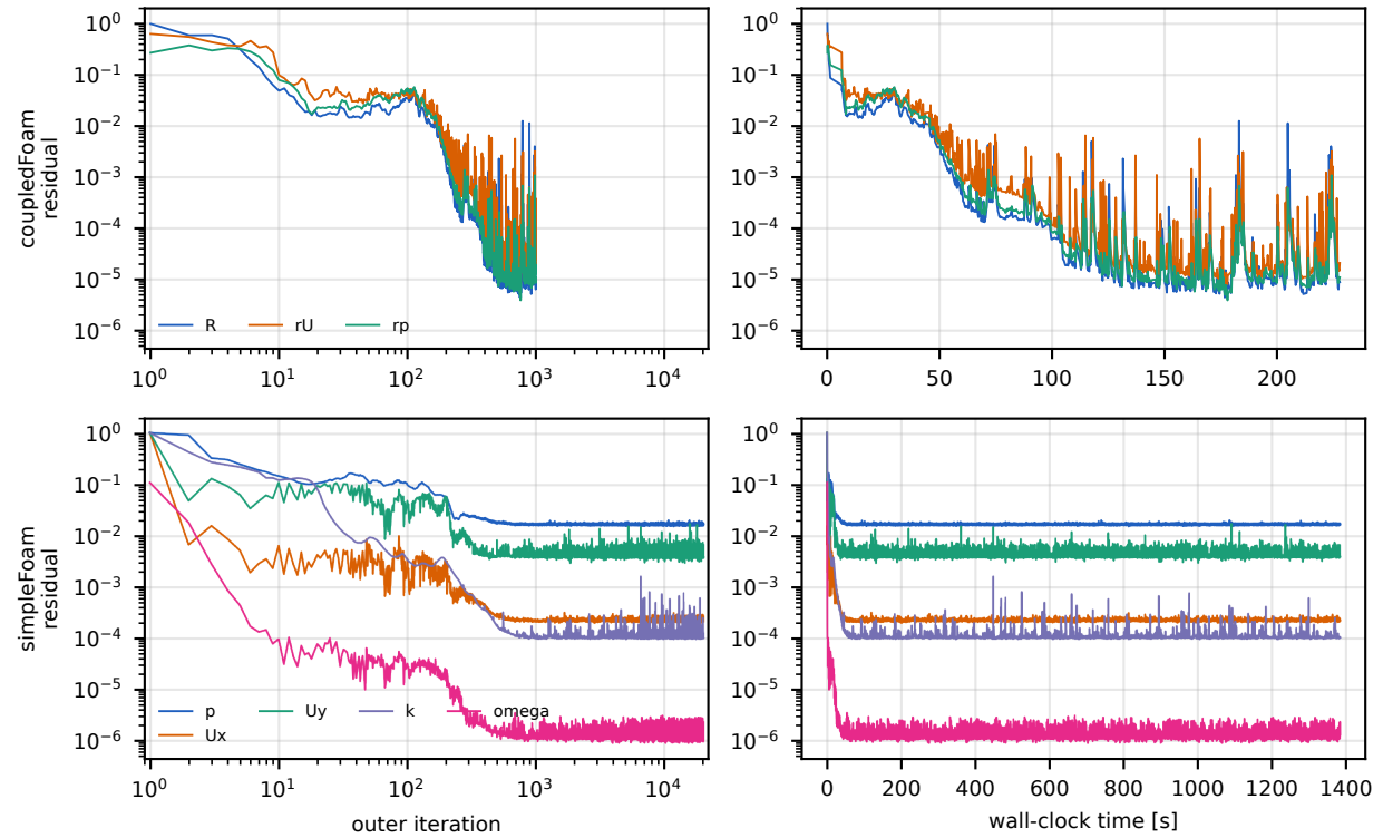
T2 backward-facing step, 1 rank: residuals (coupledFoam: combined R, momentum r_U , continuity r_p ; simpleFoam: initial residuals). Same y range; normalisations differ.
