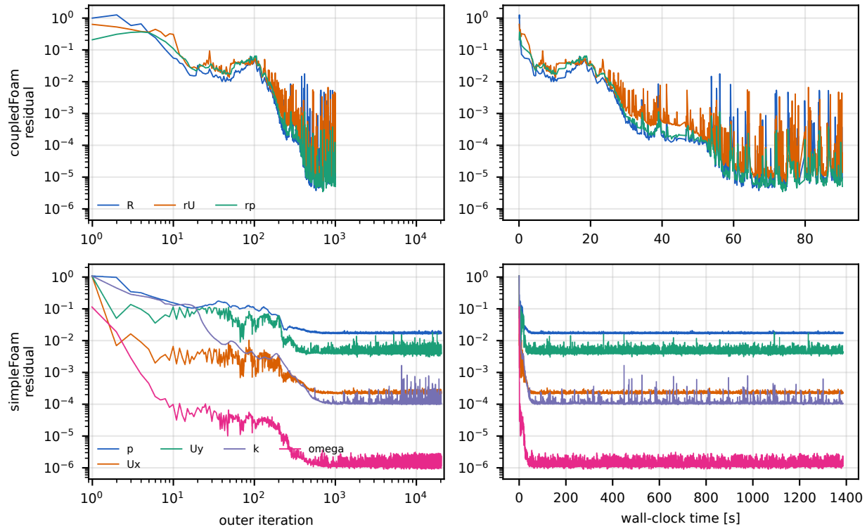
T2 backward-facing step, 4 ranks: residuals (coupledFoam: combined R , momentum r_U , continuity r_p ; simpleFoam: initial residuals). Same y range; normalisations differ.
