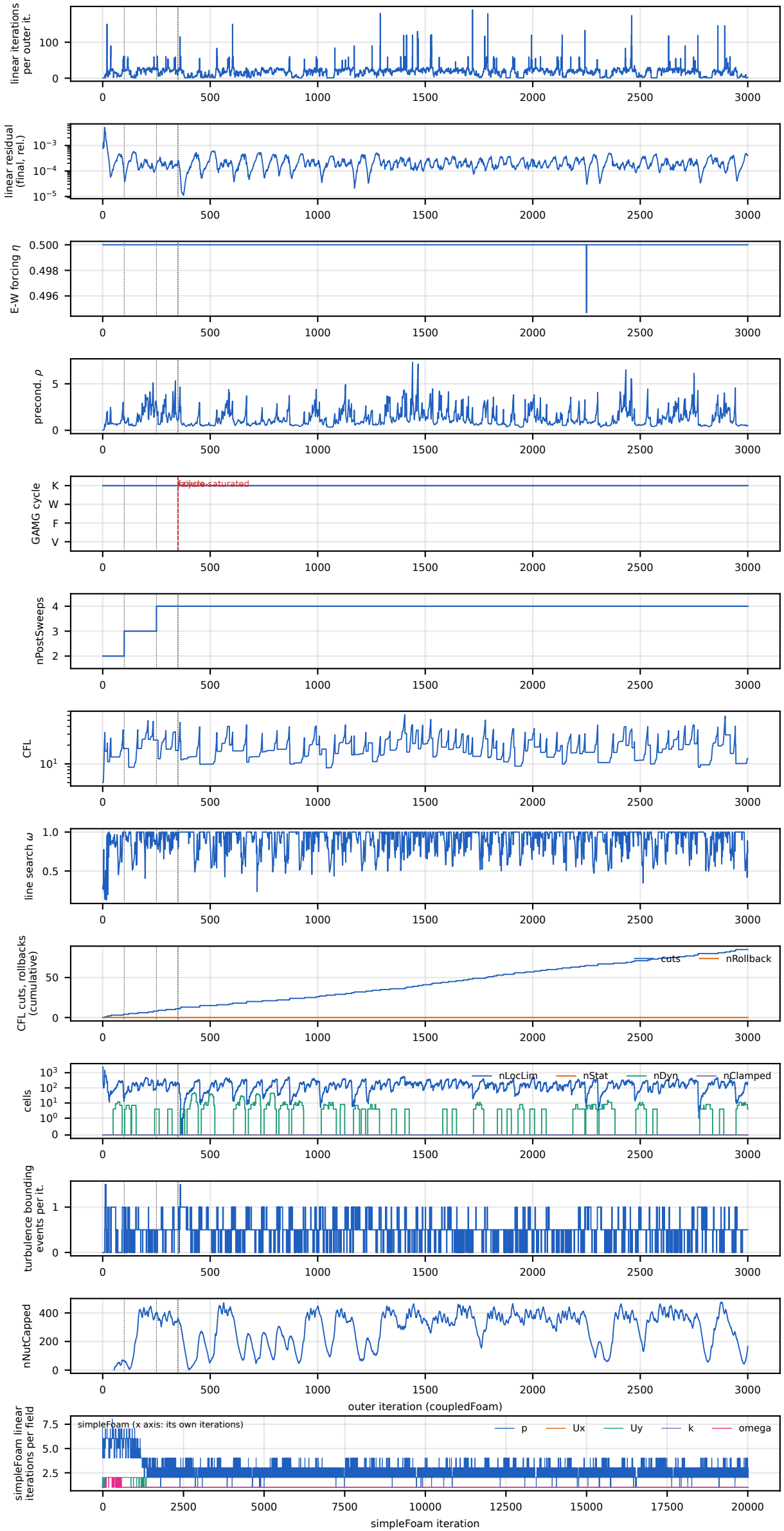
T3 airFoil2D, SST: linear solver and controls per outer iteration (dotted: GAMG autoTune events)
