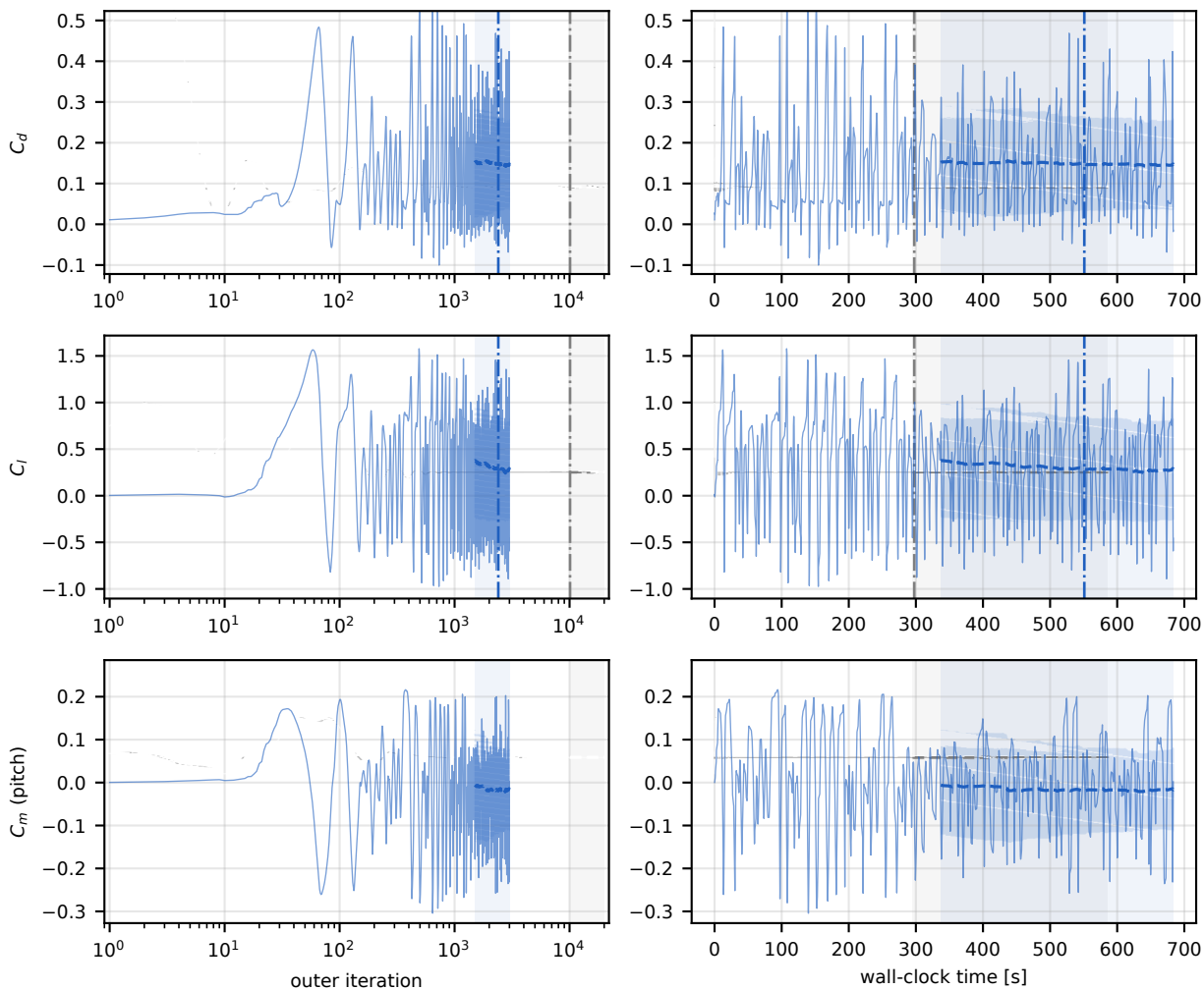
T3 airFoil2D, SST: monitored quantities (dash-dot: iterations to stationary window, D-042; shading: final averaging window)
