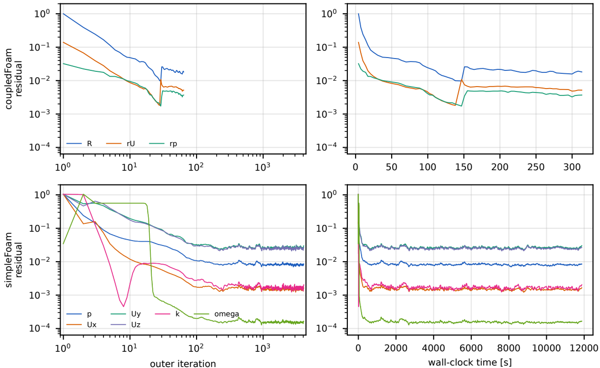
T4b motorBike, 1.70M cells, 10 ranks: residuals (coupledFoam: combined R , momentum r_U , continuity r_p ; simpleFoam: initial residuals). Same y range; normalisations differ.
