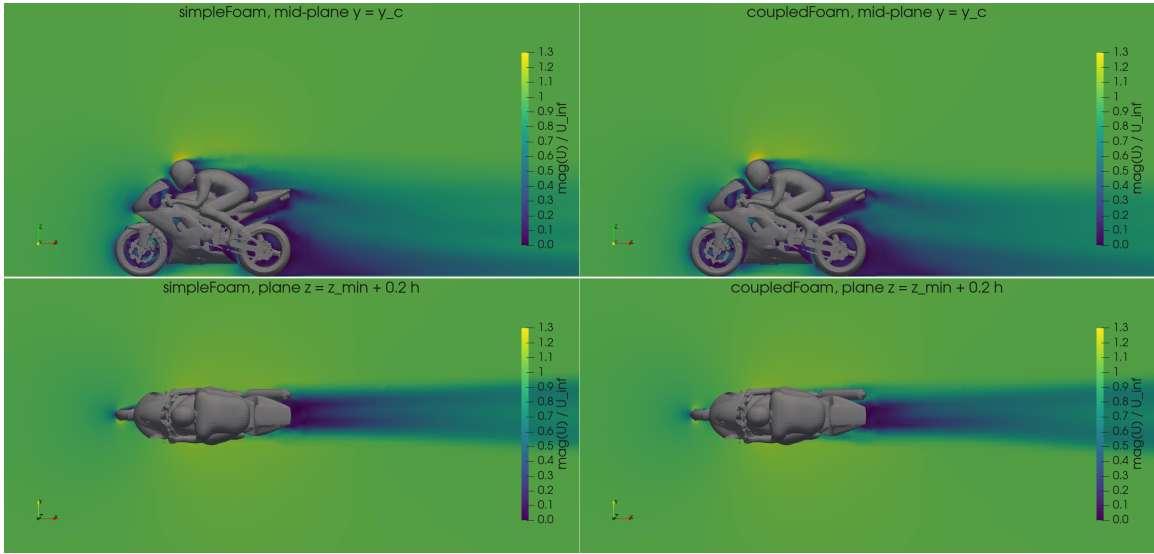
Figure 22: T4a: |\mathbf{U}|/U_\infty on the mid-plane (top) and the horizontal plane (bottom), simpleFoam (left) and coupledFoam (right).
