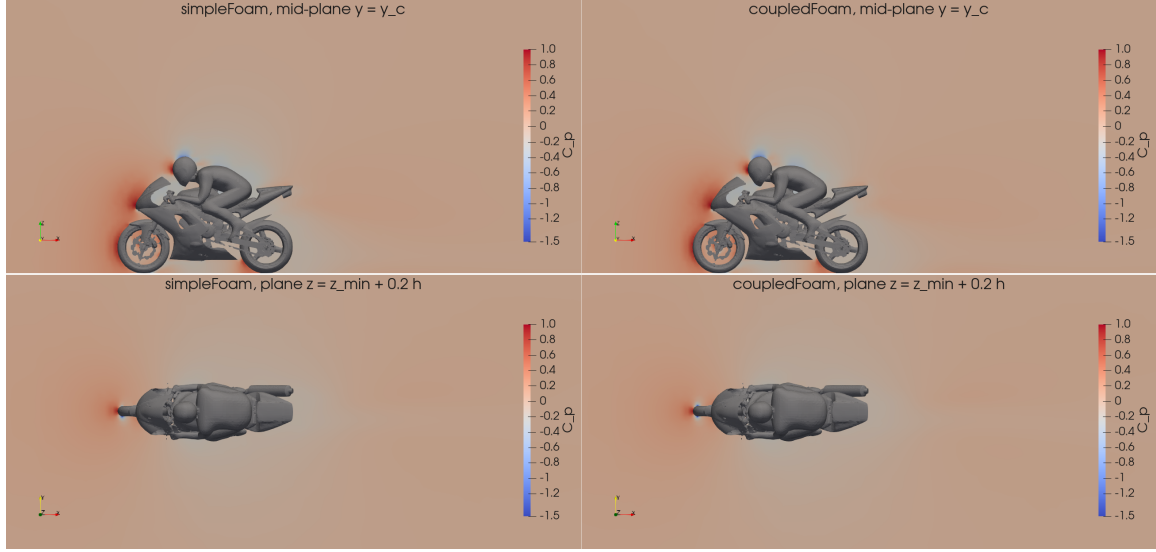
Figure 23: T4a: C_p on the mid-plane and the horizontal plane.
