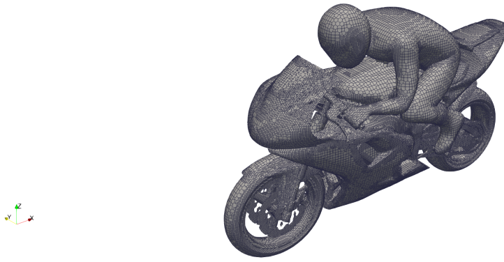
Figure 27: T4b motorBike, 1.70 M cells: body surface mesh.
