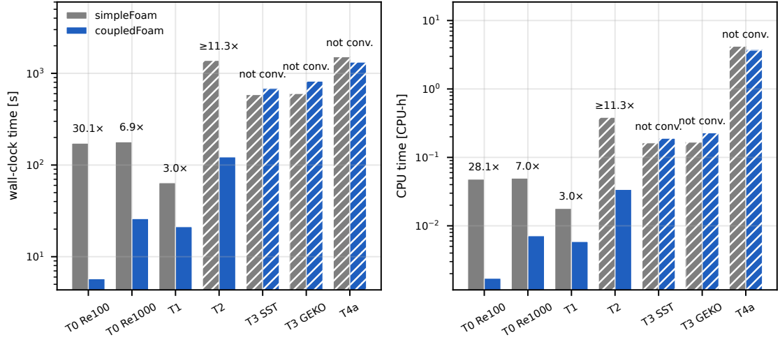
Figure 48: Wall-clock time (left) and CPU-hours (right) to convergence, simpleFoam and coupledFoam, test records, serial. Numbers: speed-up simpleFoam/coupledFoam. Hatched bars: the criterion was not reached, the bar is the whole run; \geq : lower bound.
