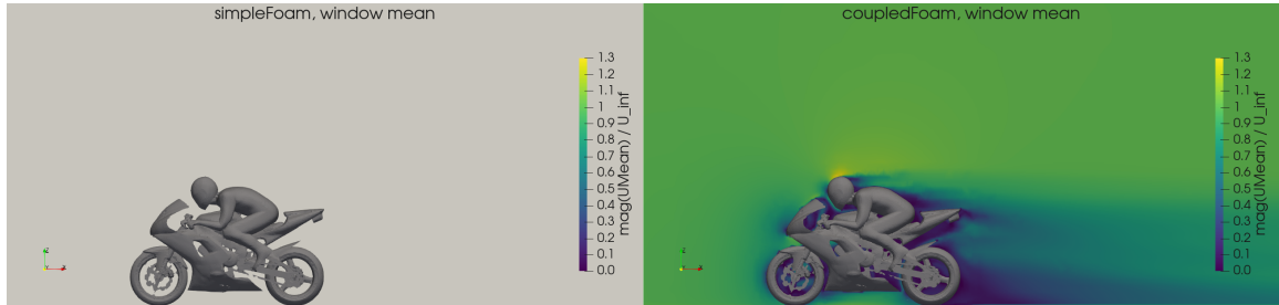
Figure 25: T4a: window-mean velocity magnitude on the mid-plane, both solvers.
