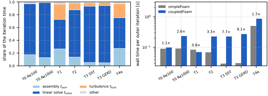
Figure 49: Time per outer iteration. Left: share of assembly, linear solve and turbulence in a coupledFoam iteration. Right: wall time per iteration of both solvers and the cost ratio coupledFoam/simpleFoam.
