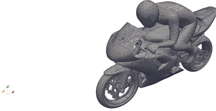
Figure 21: T4a motorBike, 354 k cells: body surface mesh.
