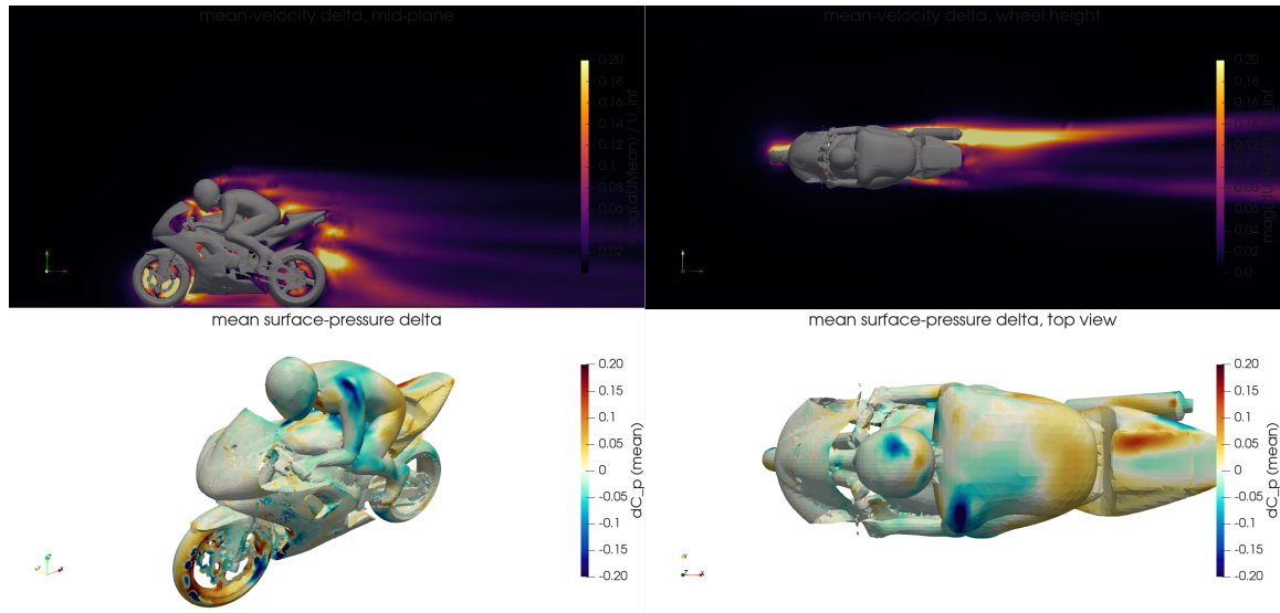
Figure 26: T4a: mean-field differences: |\Delta \mathbf{U}_{mean}|/U_{\infty} on both planes (top) and \Delta C_{p,mean} on the body (bottom).
