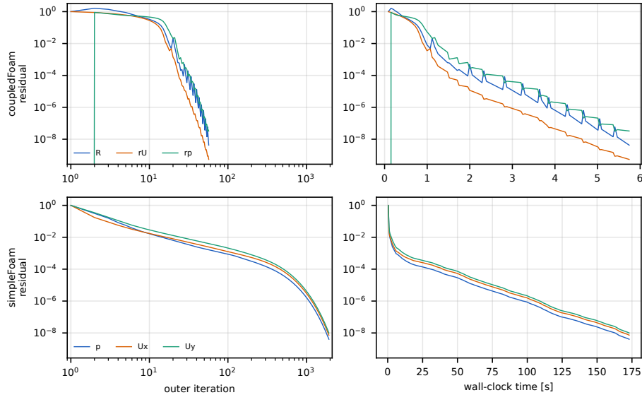
Figure 51: T0 cavity, Re 100, 1 rank: residuals per outer iteration (left) and over wall-clock time (right), coupledFoam top, simpleFoam bottom, same y range.
