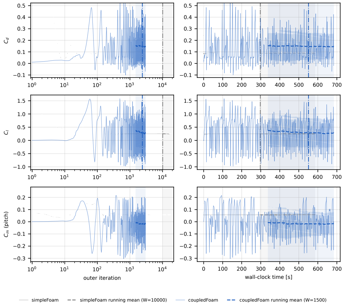
Figure 79: T3 airFoil2D, SST: monitored quantities per outer iteration (left) and over wall-clock time (right); thin: raw, dashed: running mean over the D-042 window W with \pm RMS band, shaded: final averaging window, dash-dot: iterations to a stationary window.
