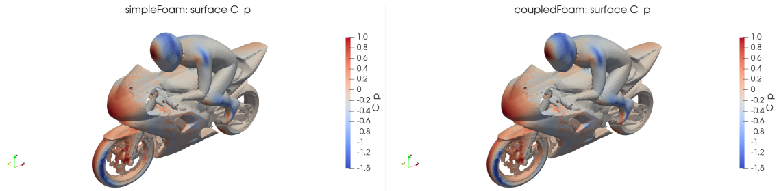
Figure 24: T4a: surface C_p on the body.
