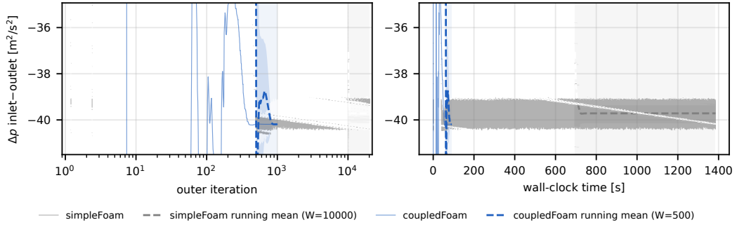
Figure 75: T2 backward-facing step, 4 ranks: monitored quantities per outer iteration (left) and over wall-clock time (right); thin: raw, dashed: running mean over the D-042 window W with \pm \text{RMS} band, shaded: final averaging window, dash-dot: iterations to a stationary window.
