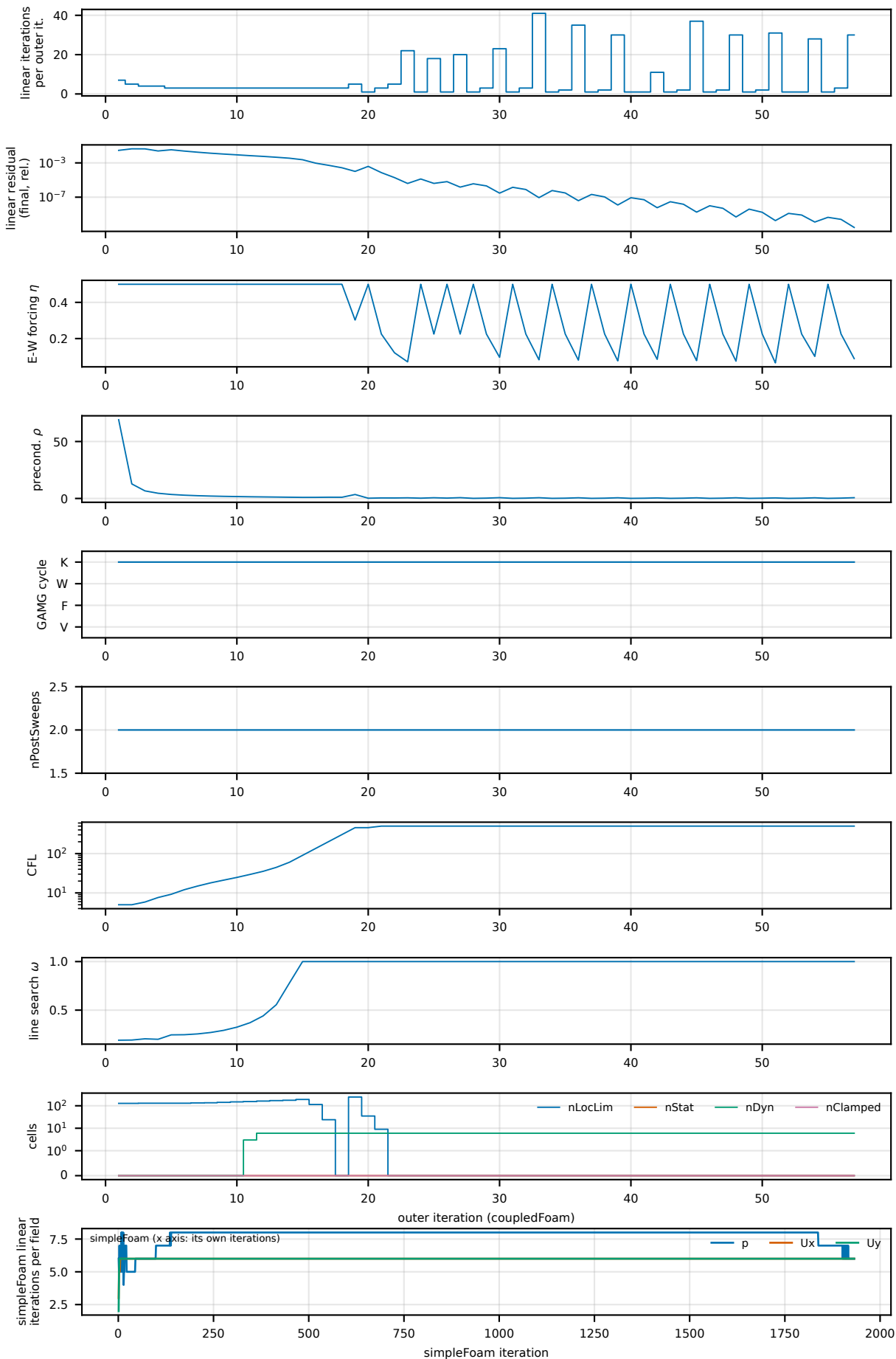
T0 cavity, Re 100, 1 rank: linear solver and controls per outer iteration (dotted: GAMG autoTune events)
