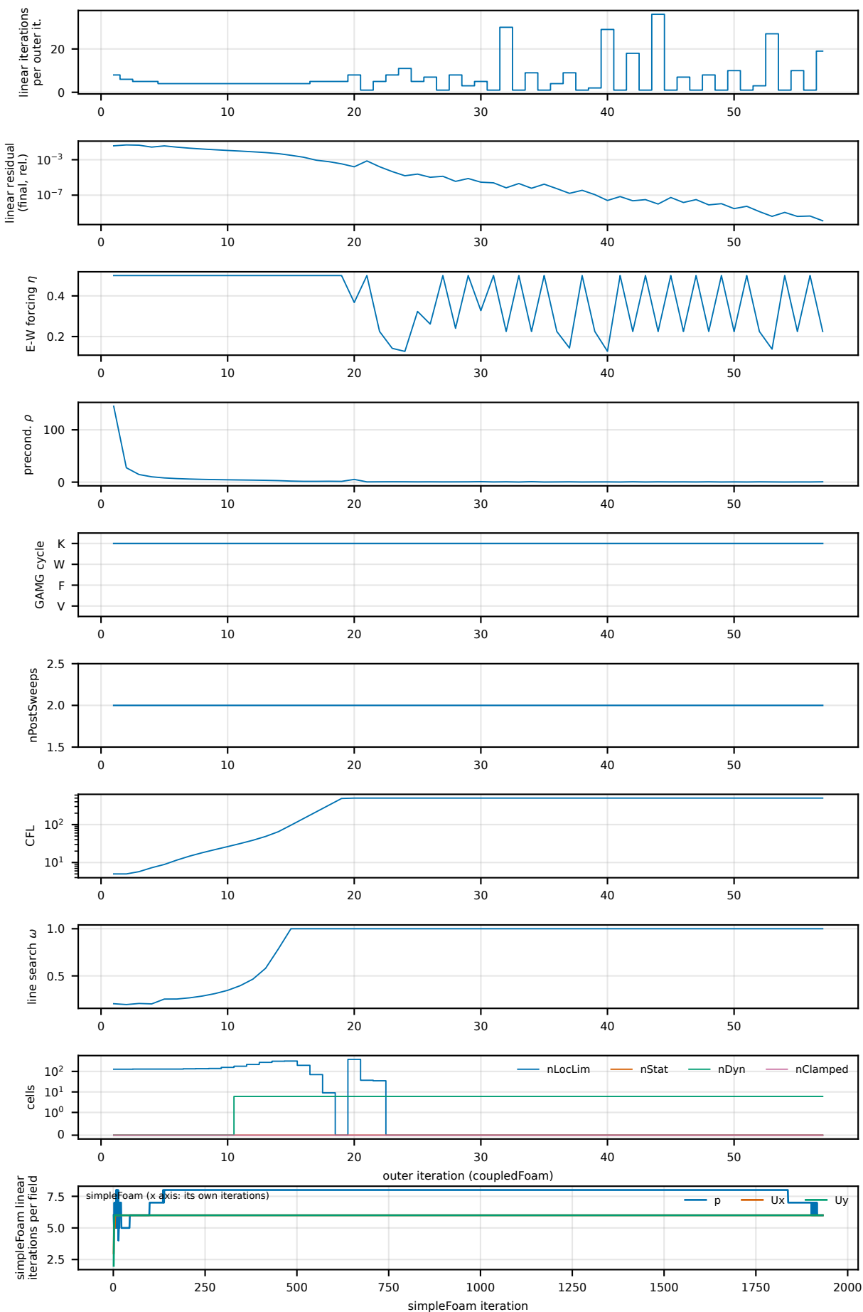
T0 cavity, Re 100, 4 ranks: linear solver and controls per outer iteration (dotted: GAMG autoTune events)
