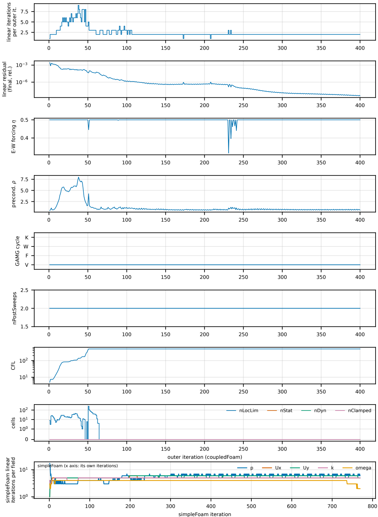
T1 pitzDaily, 1 rank: linear solver and controls per outer iteration (dotted: GAMG autoTune events)
