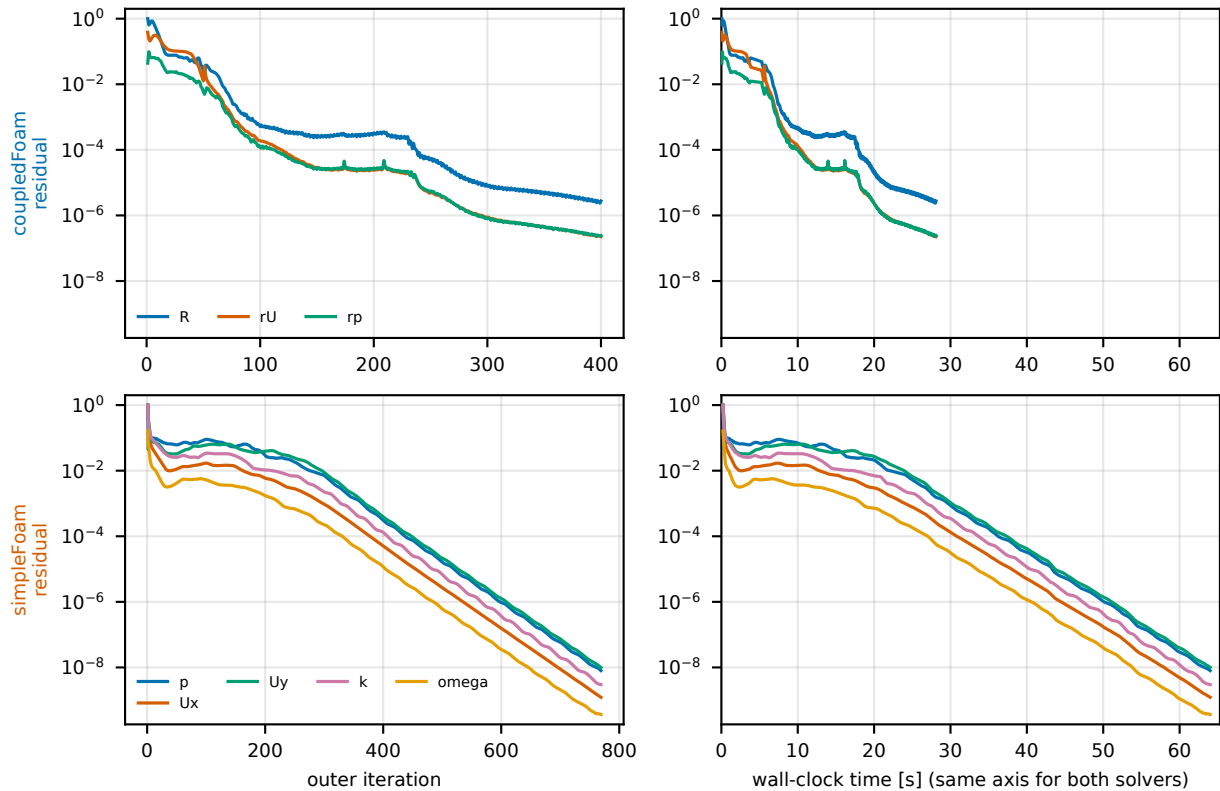
T1 pitzDaily, 1 rank: residuals (coupledFoam: combined R , momentum r_U , continuity r_p ; simpleFoam: initial residuals; long runs: band = per-bin min/max, line = bin mean). Same y range; normalisations differ.
