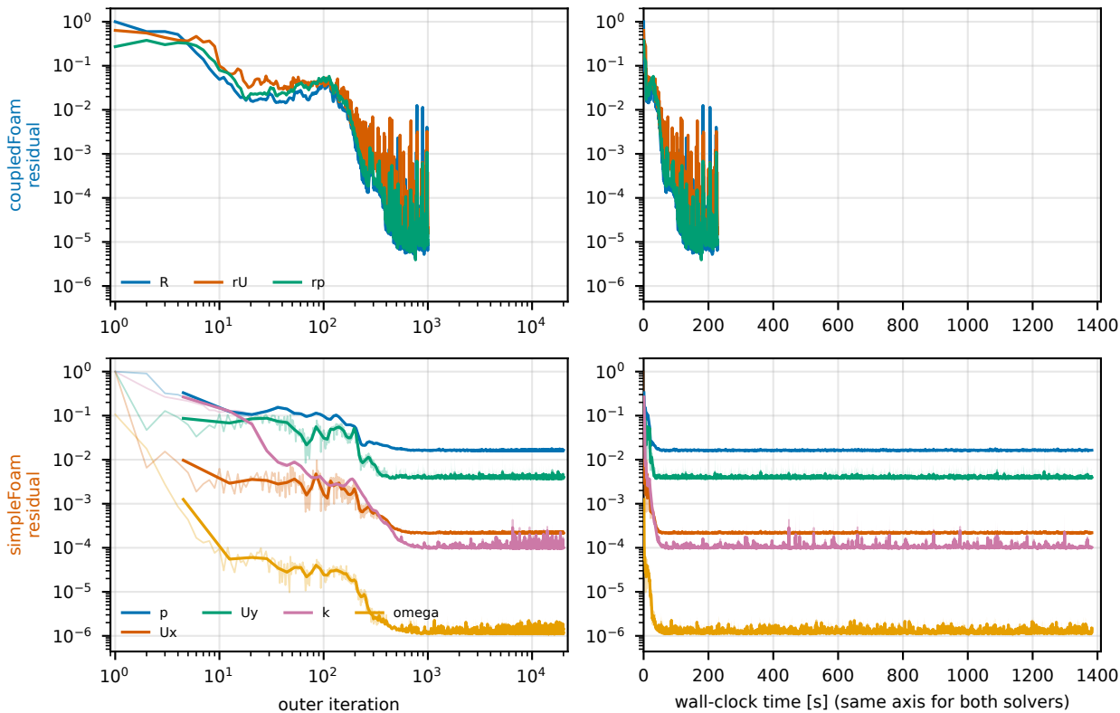
T2 backward-facing step, 1 rank: residuals (coupledFoam: combined R , momentum r_U , continuity r_p ; simpleFoam: initial residuals; long runs: band = per-bin min/max, line = bin mean). Same y range; normalisations differ.
