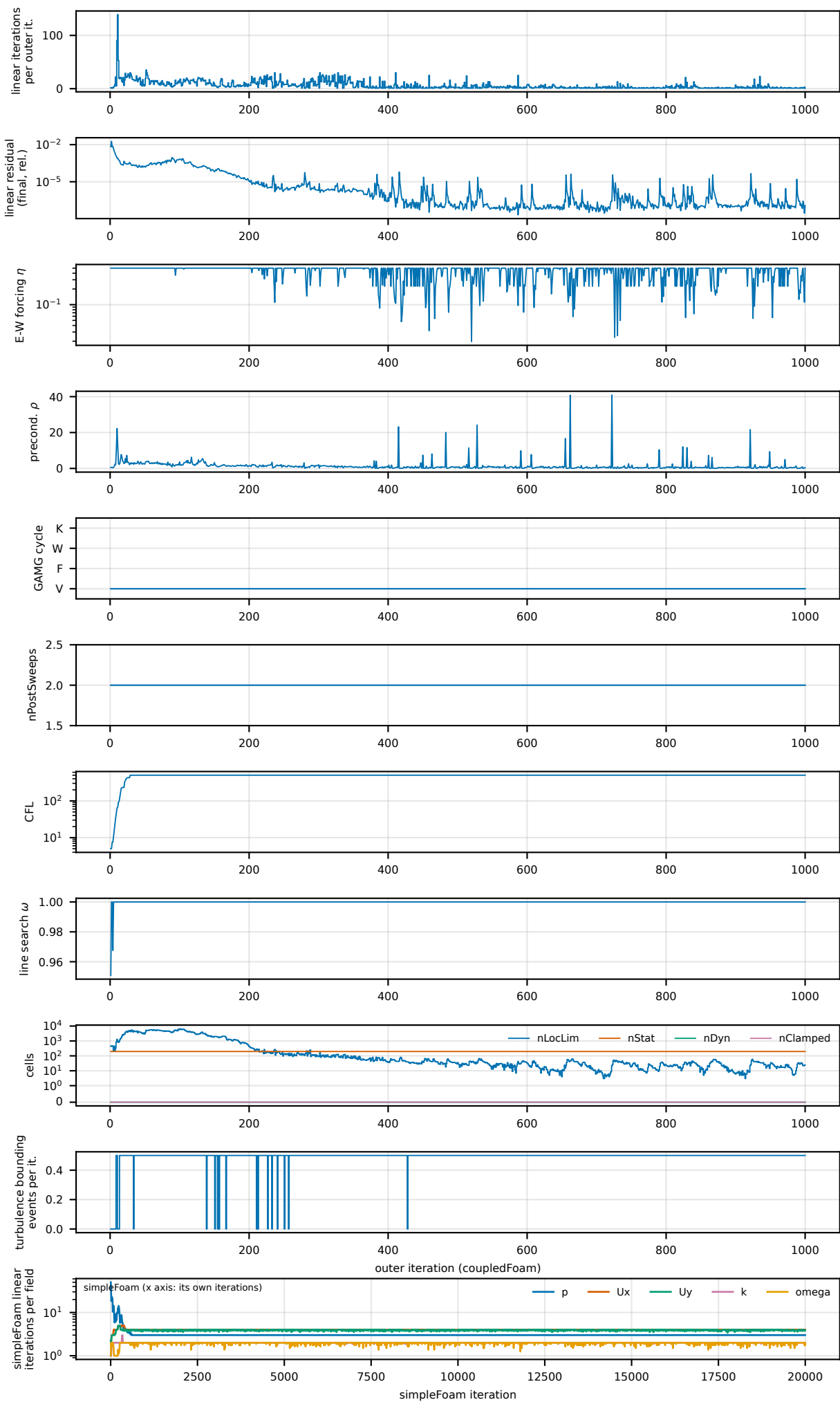
T2 backward-facing step, 4 ranks: linear solver and controls per outer iteration (dotted: GAMG autoTune events)
