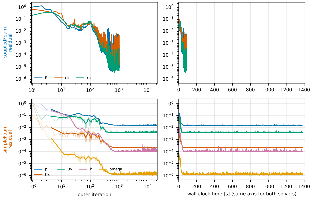
T2 backward-facing step, 4 ranks: residuals (coupledFoam: combined R , momentum r_U , continuity r_p ; simpleFoam: initial residuals; long runs: band = per-bin min/max, line = bin mean). Same y range; normalisations differ.
