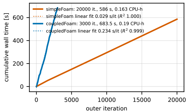
all iterations (linear axis: linear growth looks linear)
