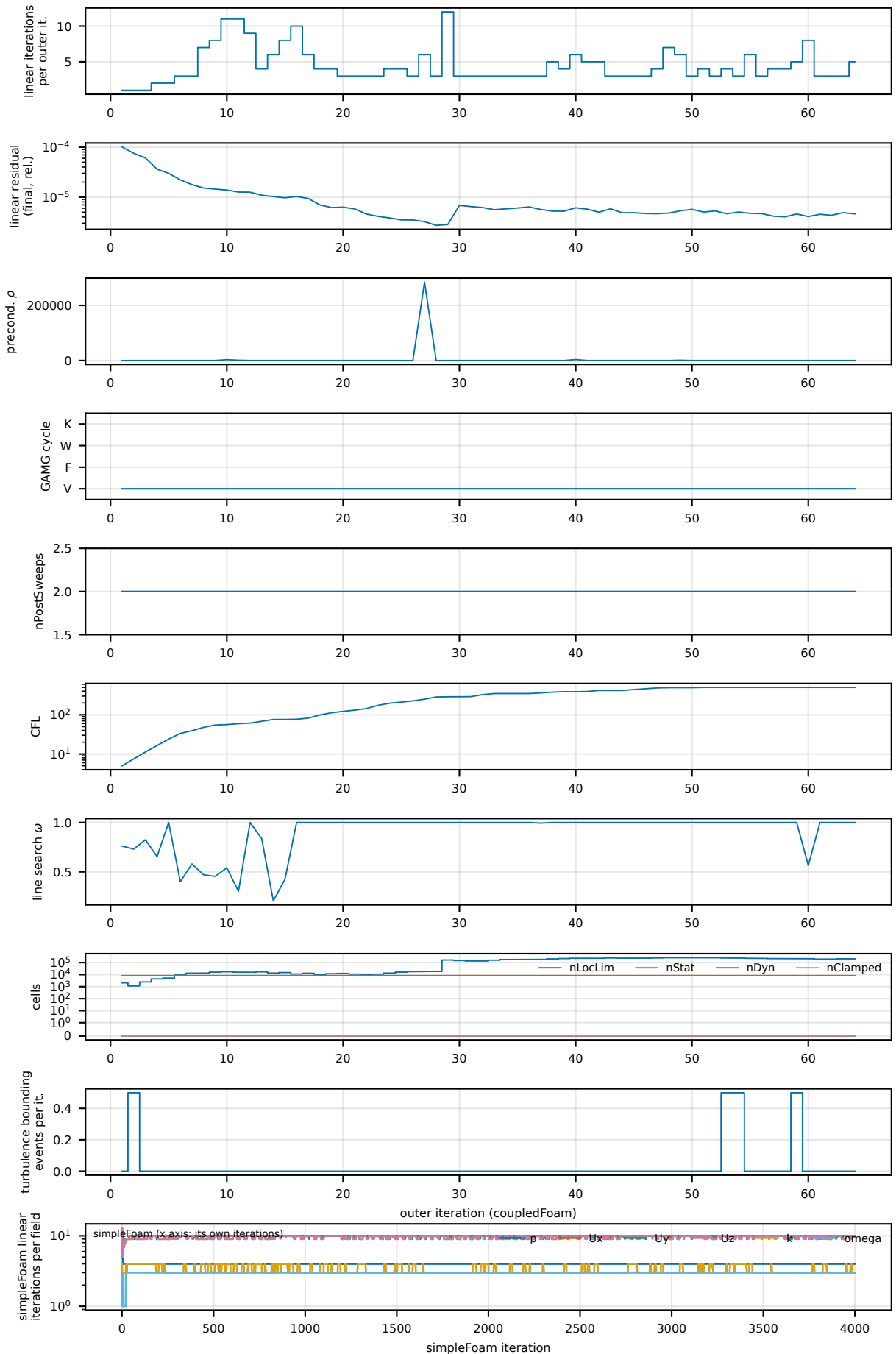
T4b motorBike, 1.70M cells, 10 ranks: linear solver and controls per outer iteration (dotted: GAMG autoTune events)
