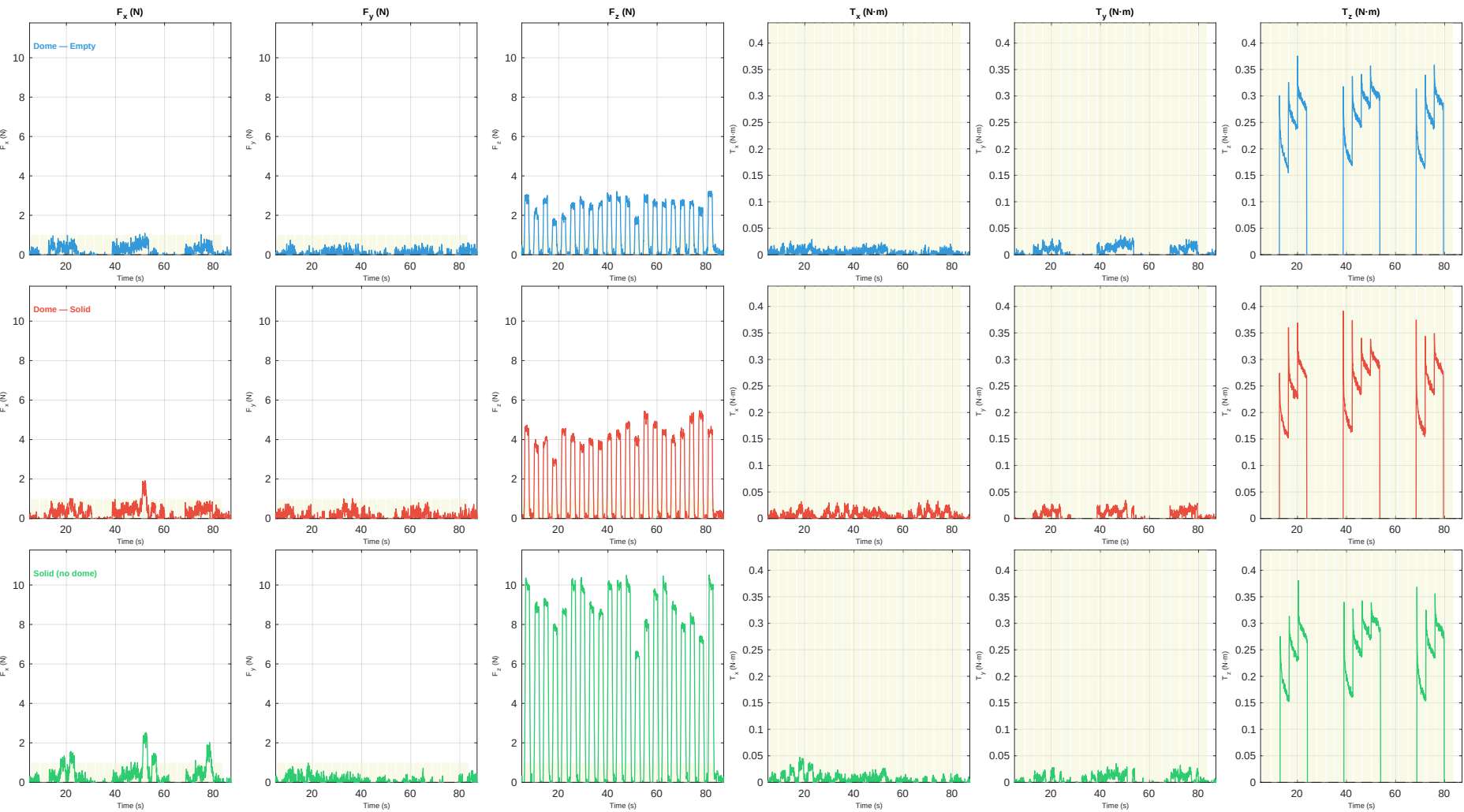
UR5 All 6 Channels — Conditioned ( t > 5 s, startup ramp excluded) Forces y_{\max} = 11.77 N | Torques y_{\max} = 0.4382 N·m | yellow = pressing
