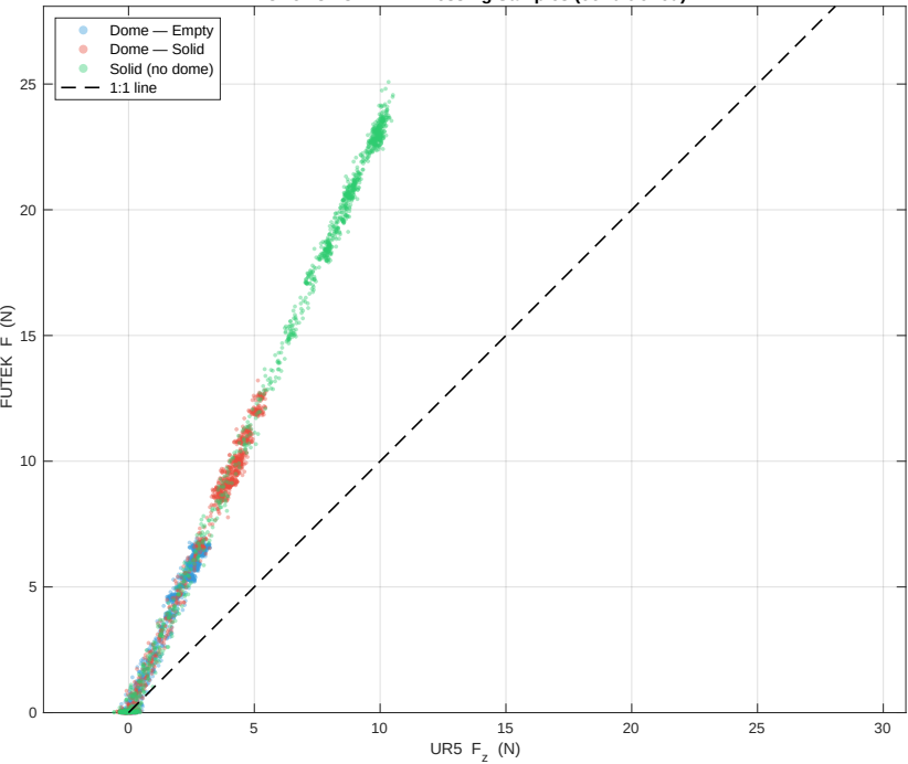
UR5 vs FUTEK — Pressing Samples (conditioned)
