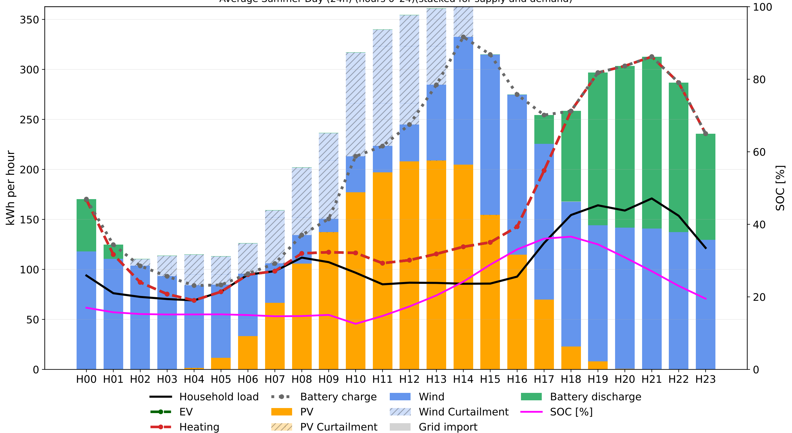
Average Summer Day (24h) (hours 0-24)(stacked for supply and demand)
