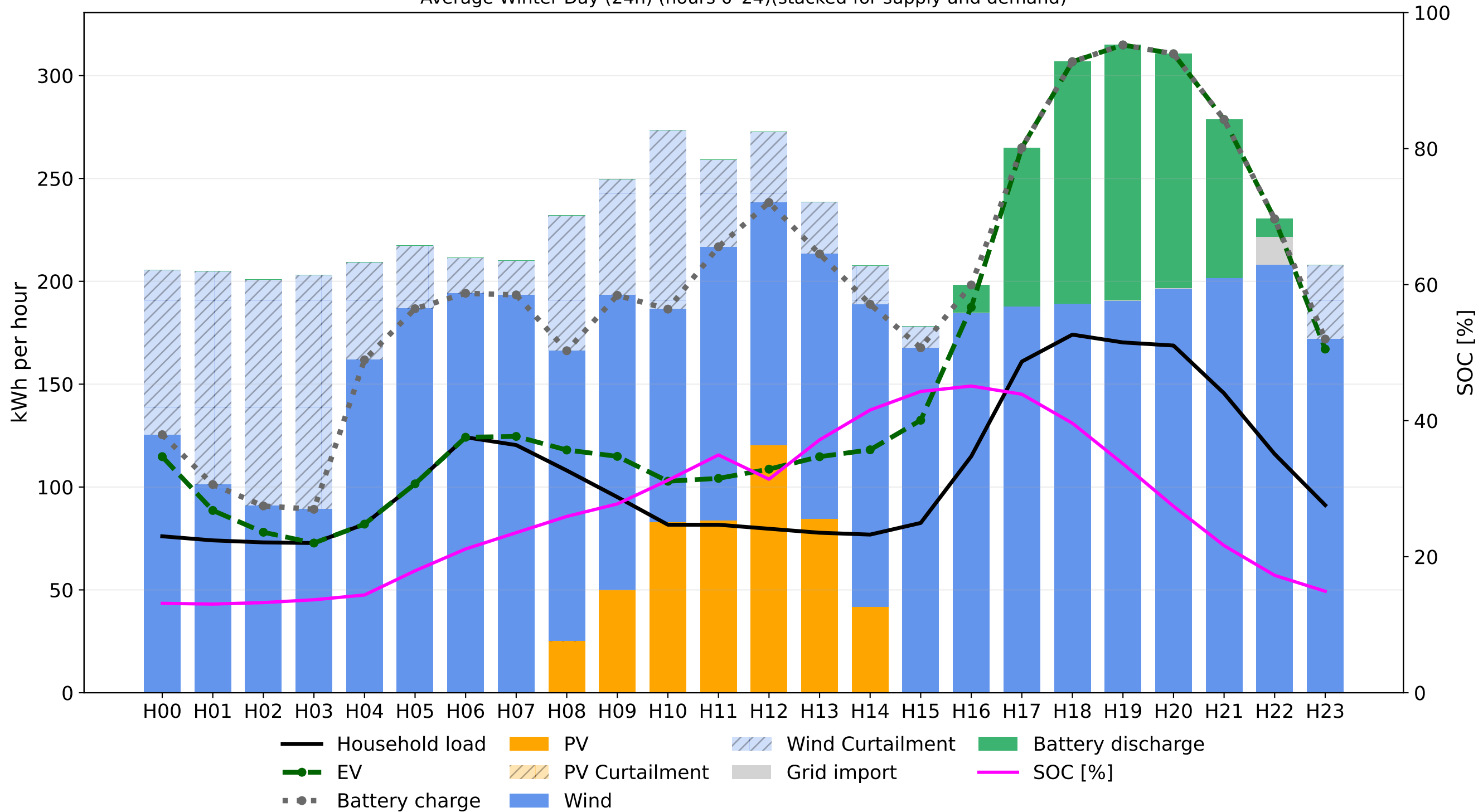
Average Winter Day (24h) (hours 0-24)(stacked for supply and demand)
