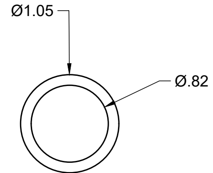
CROSS-SECTION Scale = 1:1
