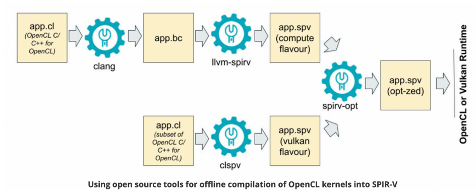
Fig. 7.2: Offline Compilation of OpenCL Kernels into SPIR-V Using Open Source Tooling 11
