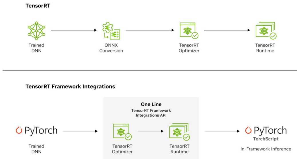
Fig. 7.8: Tensor-RT
