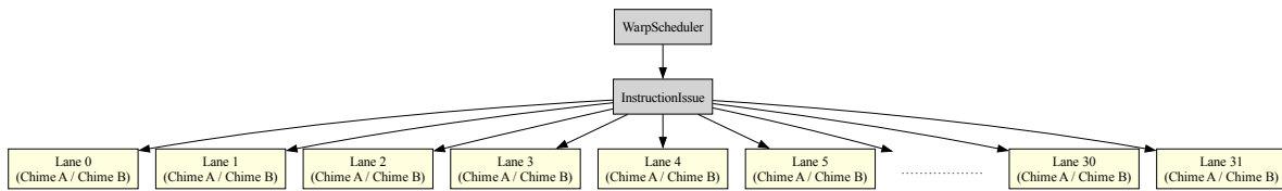
Fig. 6.14: In dual-issue mode , Chime A carries floating-point data while Chime B carries integer data—both issued by the same CUDA thread. In contrast, under time-sliced execution , Chime A and Chime B carry either floating-point or integer data independently, and are assigned to separate CUDA threads.
