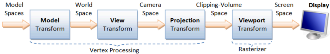
Fig. 4.18: Coordinates Transform Pipeline Page 32, 4
