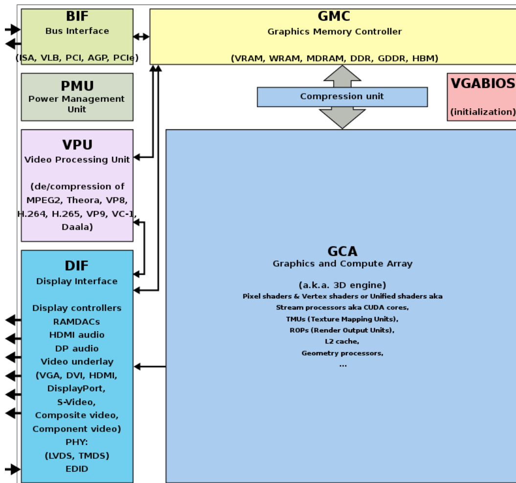
Fig. 6.2: Components of a GPU: GPU has accelerated video decoding and encoding Page 103, 2
