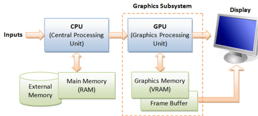
Fig. 6.1: Computer Graphics Hardware (figure from book Page 103, 1 )
