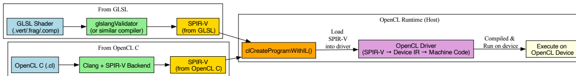
Fig. 7.4: Compiling and Deploying GPU Code from GLSL, Vulkan, and OpenCL
