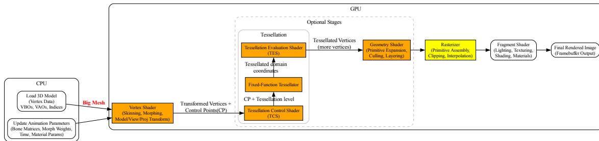
Fig. 5.15: CPU and GPU Traditional Pipeline For Shaders
