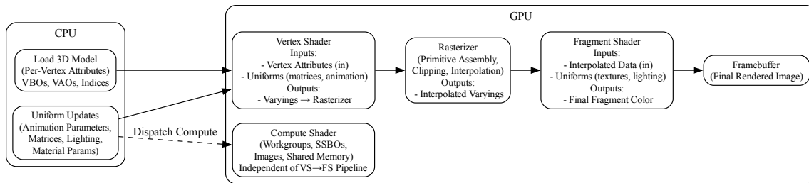
Fig. 5.19: Shaders input and output
