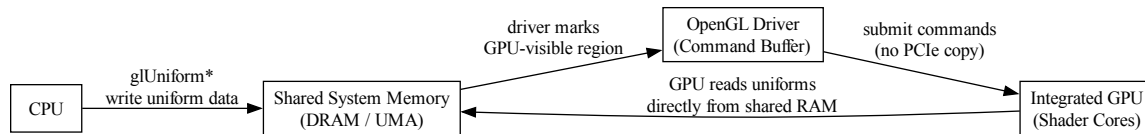
Fig. 6.19: CPU send Uniform Updates Data to iGPU for rendering
