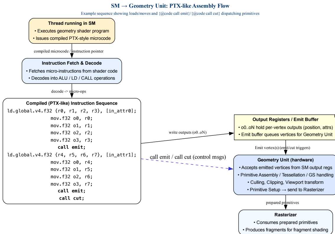
Fig. 6.24: Fetch a sequence of Geometry instructions and pass to Geometry Unit
