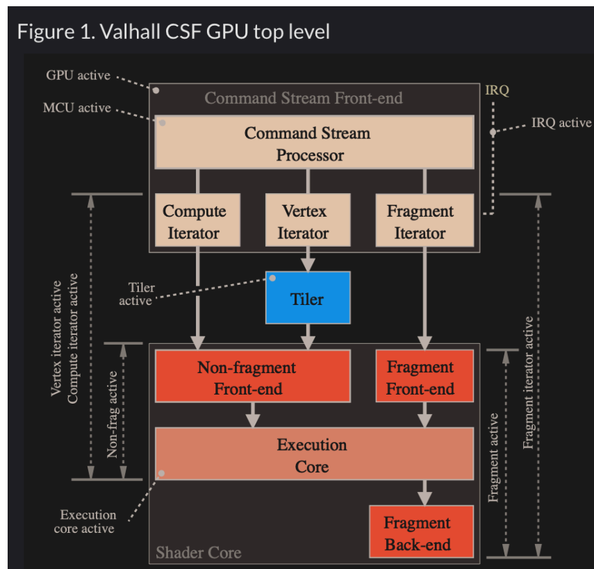
Fig. 3.3: MCU and specific HW circuits to speedup the processing of CSF (Command Stream Fronted) Page 21, 5 .
