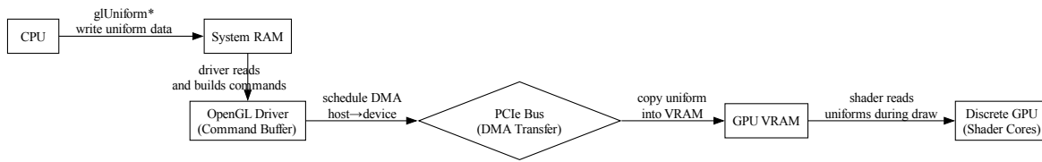
Fig. 6.18: CPU send Uniform Updates Data to dGPU for rendering
