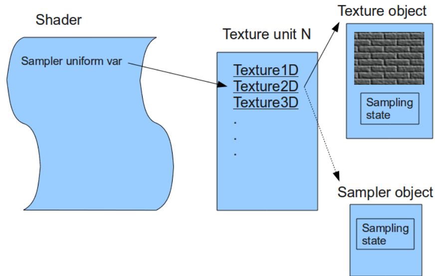
Fig. 5.20: Relationships between the texturing concept 35 .
