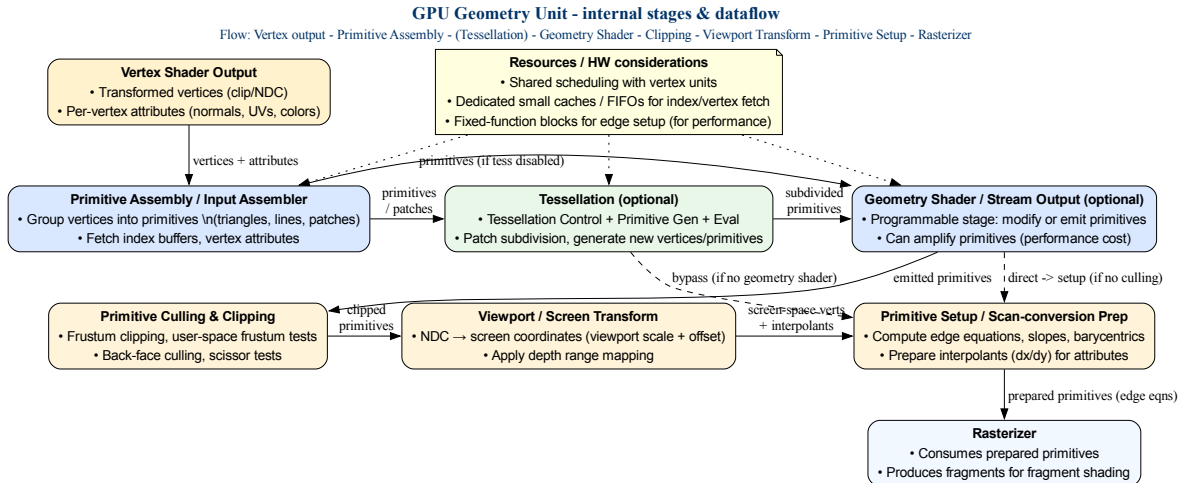
Fig. 6.26: Geometry Unit with its sub-functions (assembly, tessellation, clipping, viewport transform, etc.)
