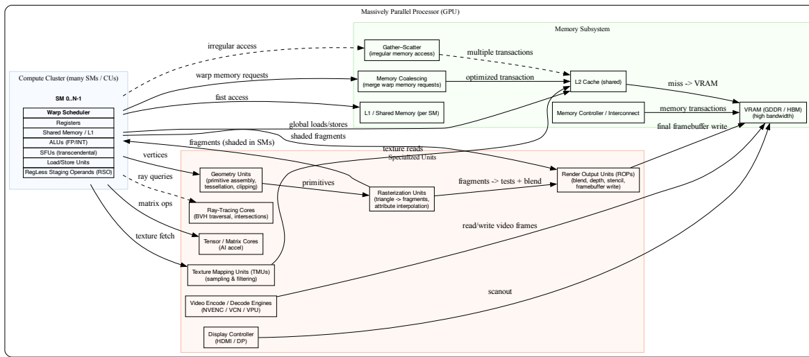
Fig. 6.3: Components of a GPU: SIMD/SIMT + several specialized processing units
