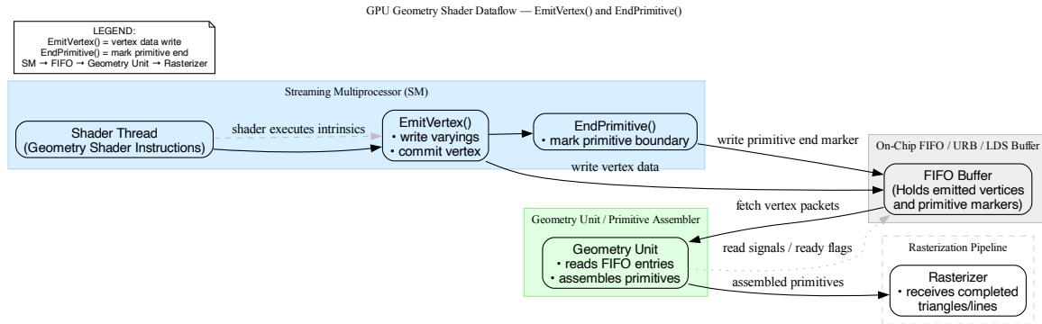
Fig. 6.23: Micro-level flow: SM → Geometry Unit via Emit/Cut
