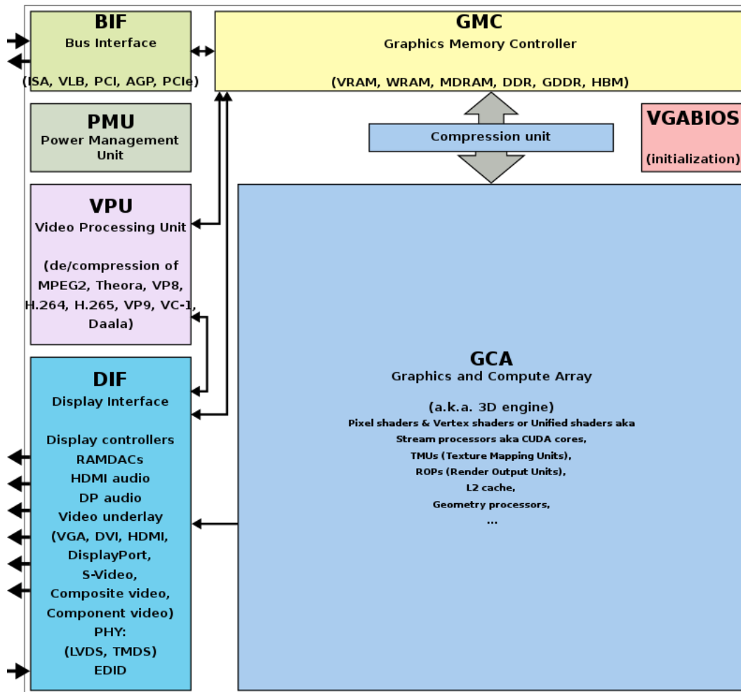
Fig. 6.2: Components of a GPU: GPU has accelerated video decoding and encoding Page 101, 2
