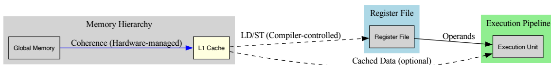
Fig. 6.18: Operand Delivery in Traditional GPU (Traditional Model: Register File + L1 Cache)
