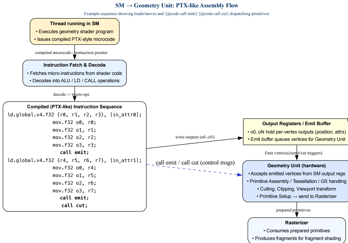
Fig. 6.22: Fetch a sequence of Geometry instructions and pass to Geometry Unit
