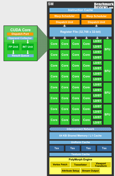
Fig. 6.7: SM figure from websites 8,9 .
