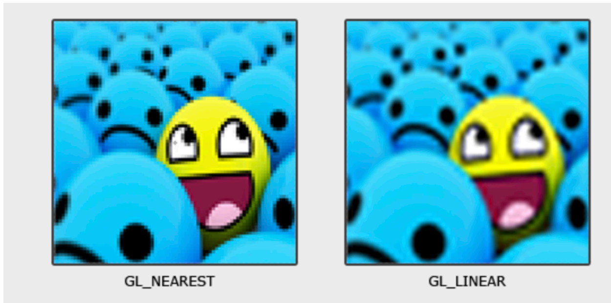
Fig. 6.31: Texture Filter: GL_NEAREST has sharp color and jagged edge Page 134, 27
