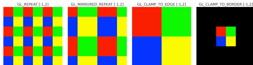
Fig. 6.27: Texture Warpping
