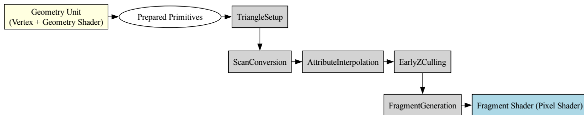
Fig. 6.25: Rasterization pipeline
