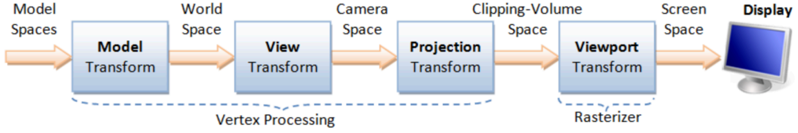
Fig. 4.19: Coordinates Transform Pipeline Page 32, 4
