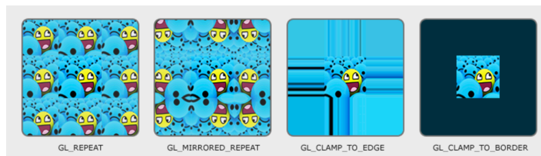
Fig. 6.28: Texture Warpping 27
