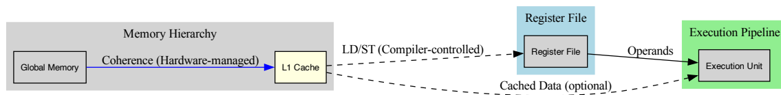
Fig. 2.71: Operand Delivery in Traditional GPU (Traditional Model: Register File + L1 Cache)
