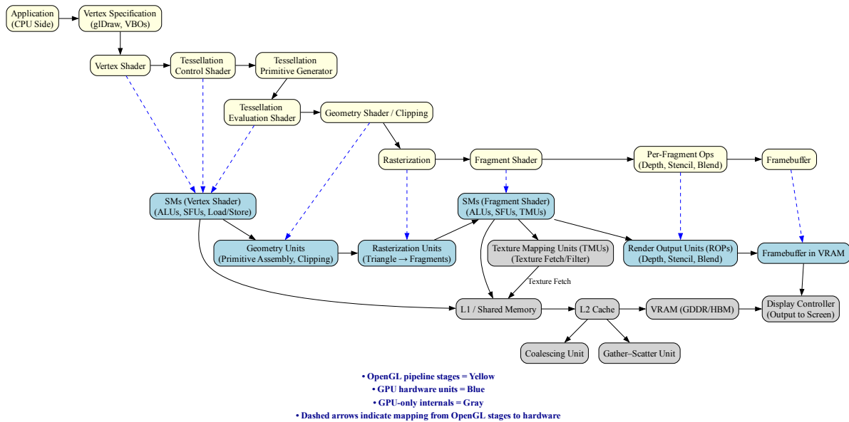
Fig. 2.73: The stages of OpenGL pipeline and GPU's acceleration components
