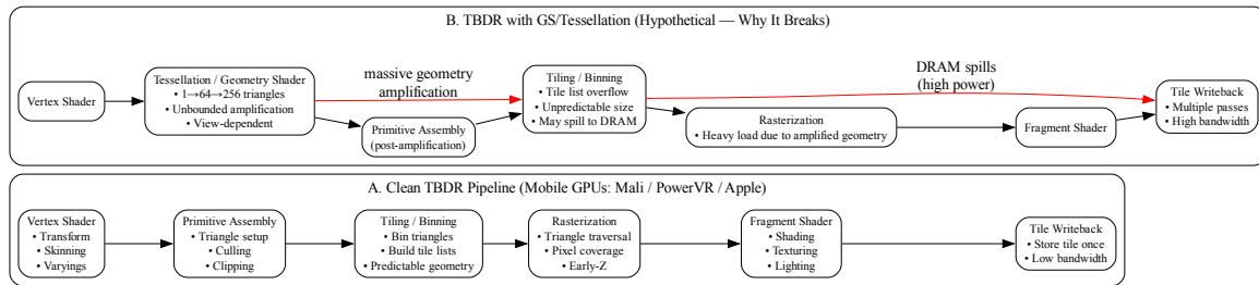
Fig. 2.43: CPU and GPU Pipeline For Shaders in Mobile Device
