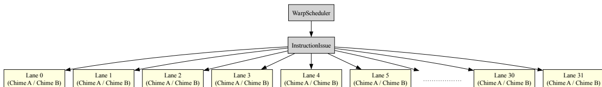
Fig. 2.67: In dual-issue mode , Chime A carries floating-point data while Chime B carries integer data—both issued by the same CUDA thread. In contrast, under time-sliced execution , Chime A and Chime B carry either floating-point or integer data independently, and are assigned to separate CUDA threads.
