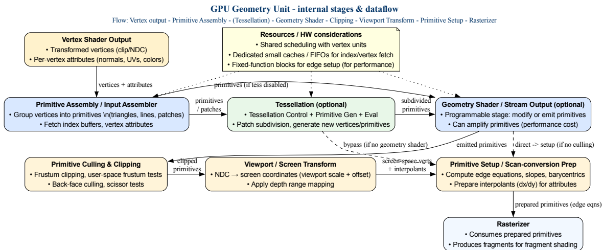
Fig. 2.77: Geometry Unit with its sub-functions (assembly, tessellation, clipping, viewport transform, etc.)
