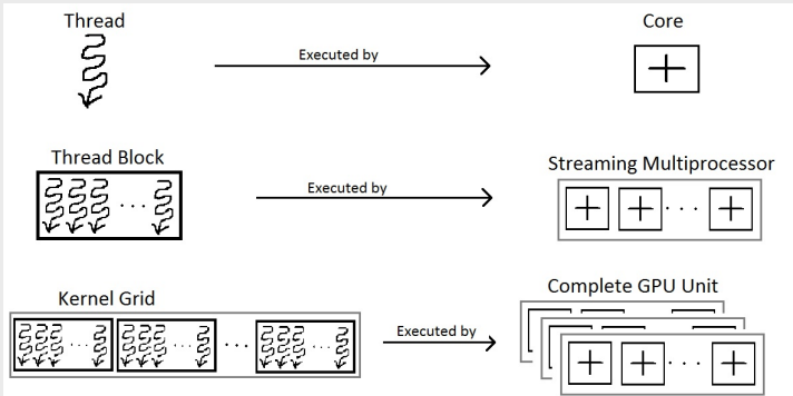
Fig. 2.61: SM select Thread Blocks to run 100 .
