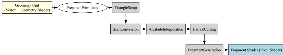
Fig. 2.78: Rasterization pipeline
