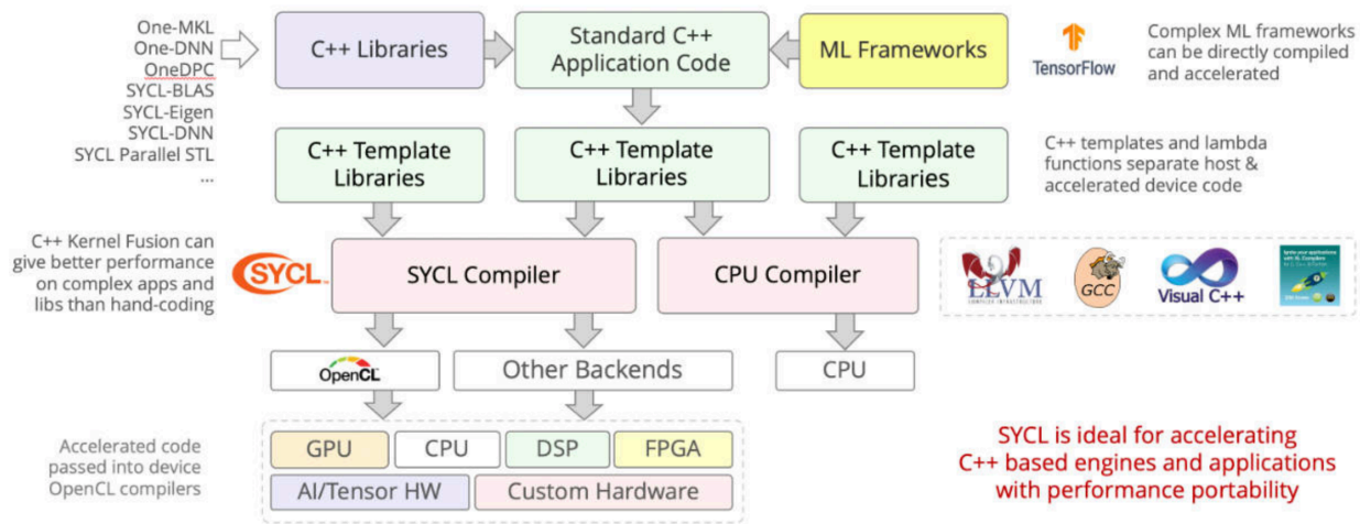
Fig. 2.97: SYCL = C++ template and compiler for Data Parallel Applications on AI on CPUs, GPUs and HPGAs.
