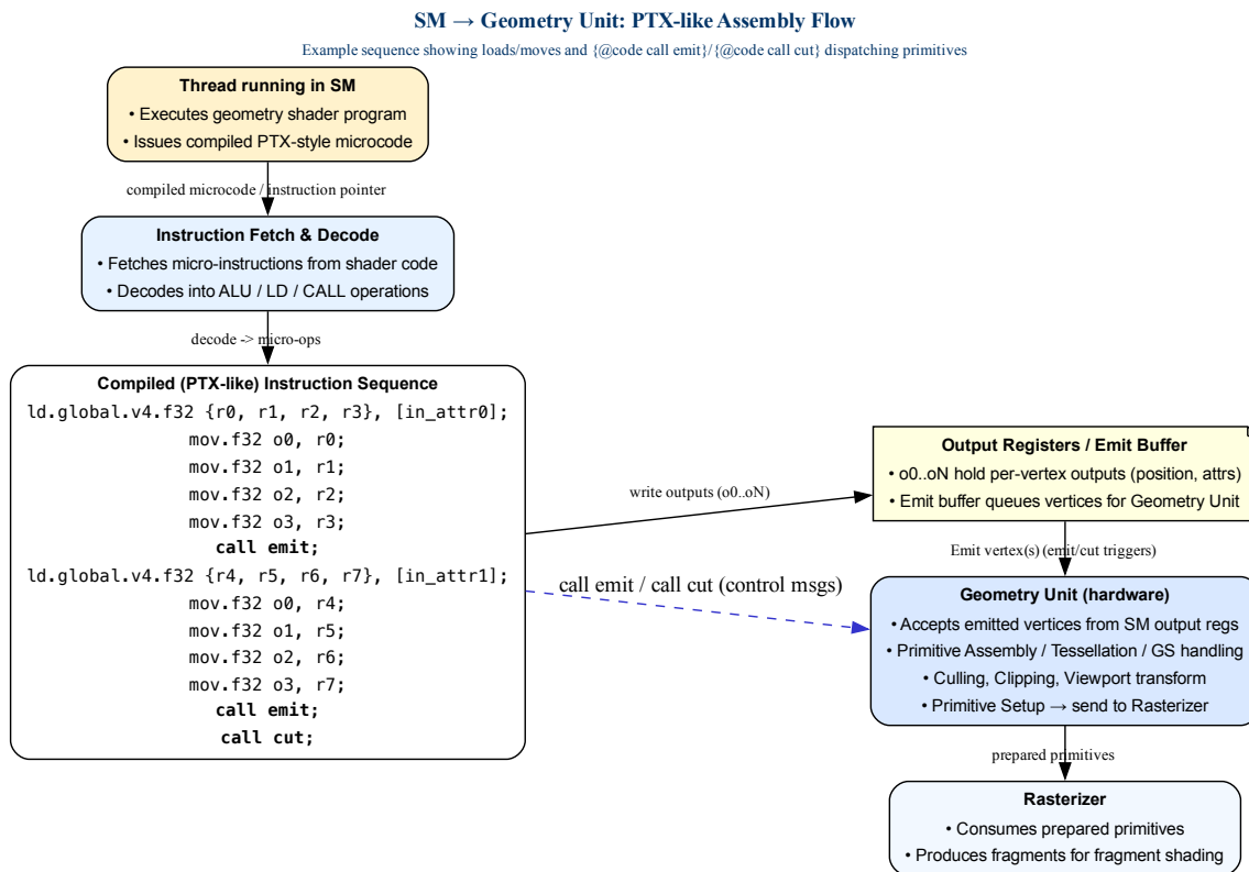
Fig. 2.75: Fetch a sequence of Geometry instructions and pass to Geometry Unit
