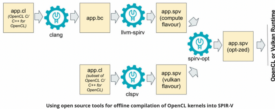
Fig. 2.87: Offline Compilation of OpenCL Kernels into SPIR-V Using Open Source Tooling 113
