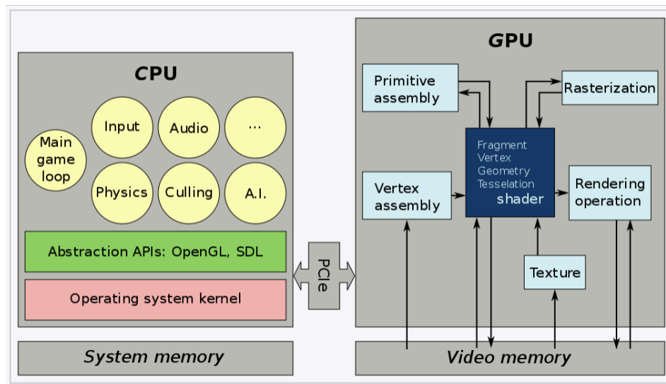
Fig. 2.6: OpenGL and Vulkan are both rendering APIs. In both cases, the GPU executes shaders, while the CPU executes everything else Page 22, 11 .
