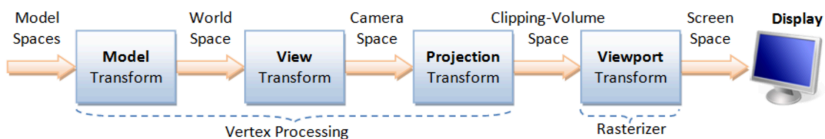
Fig. 2.15: Coordinates Transform Pipeline Page 5, 1
