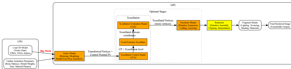
Fig. 2.47: CPU and GPU Traditional Pipeline For Shaders
