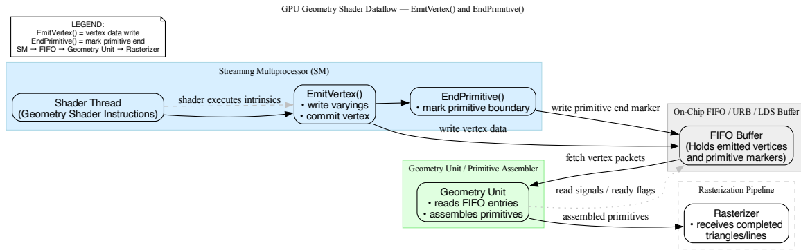
Fig. 2.76: Micro-level flow: SM → Geometry Unit via Emit/Cut
