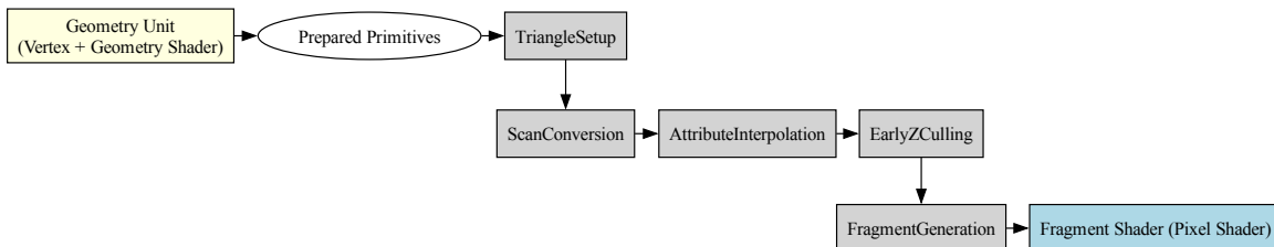
Fig. 6.27: Rasterization pipeline
