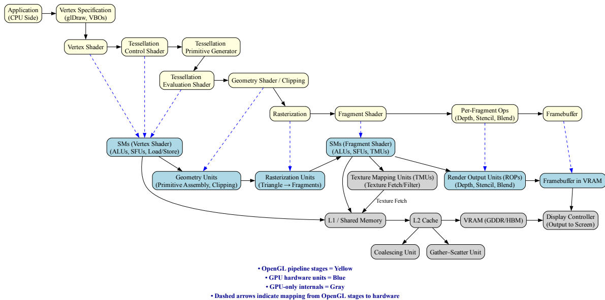
Fig. 6.4: The stages of OpenGL pipeline and GPU's acceleration components
