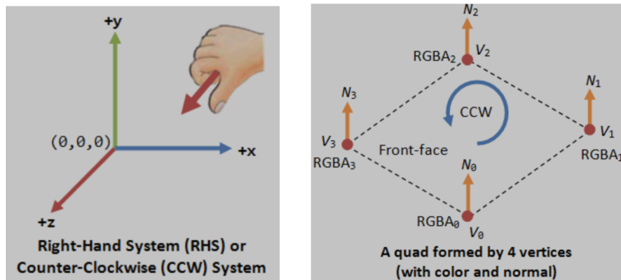
Fig. 4.14: OpenGL pointing outwards, indicating the outer surface ( z axis is + )
