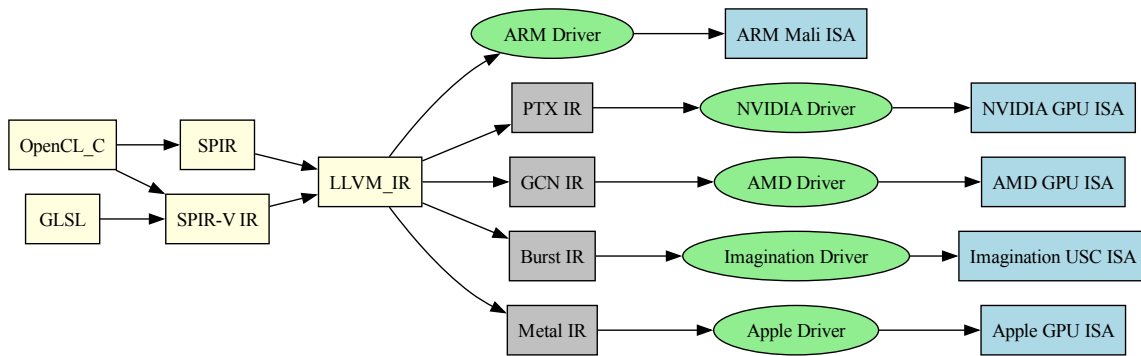
Fig. 7.6: Graphics and OpenCL Compiler IR Conversion Flow
