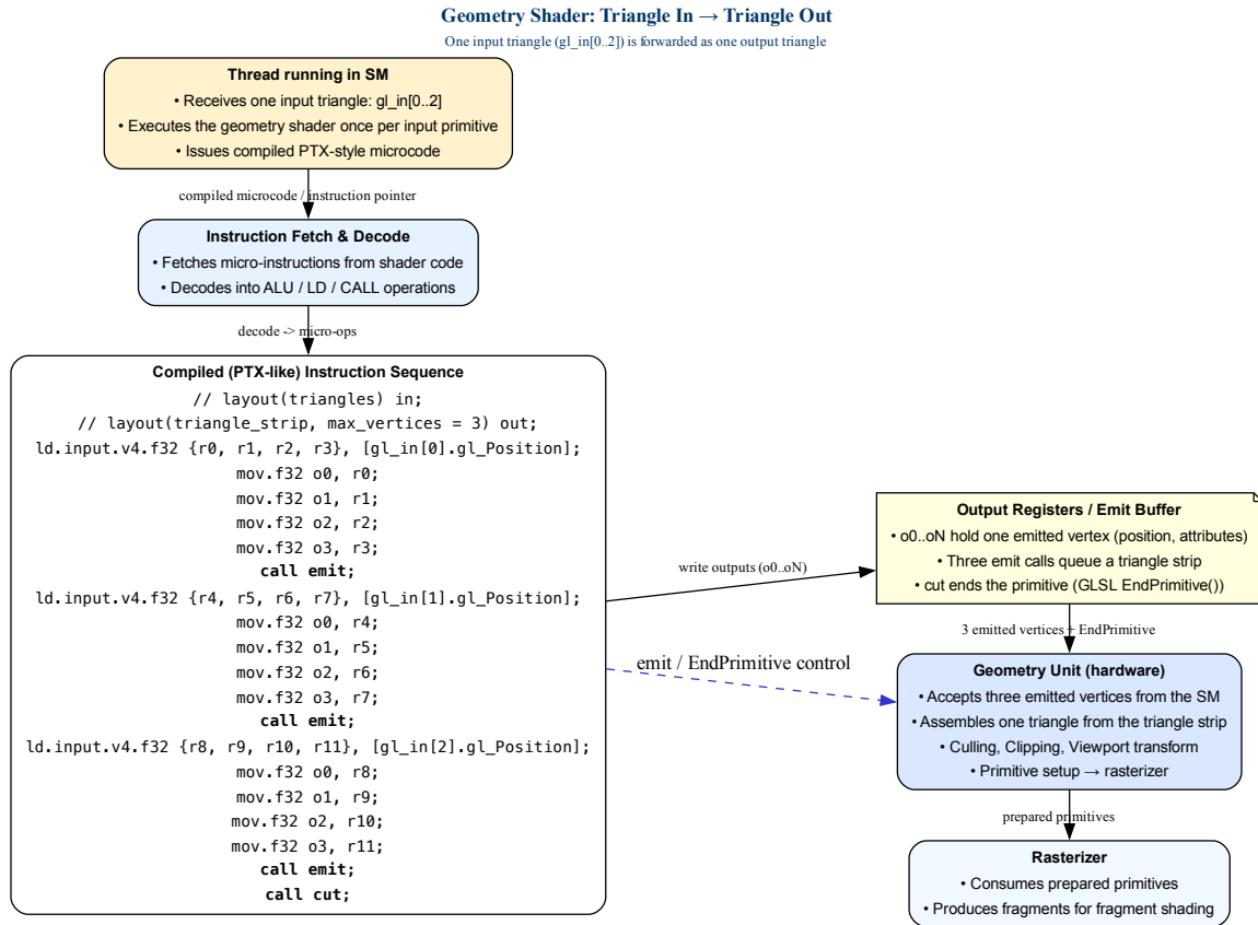
Fig. 6.24: Fetch a sequence of Geometry instructions and pass to Geometry Unit
