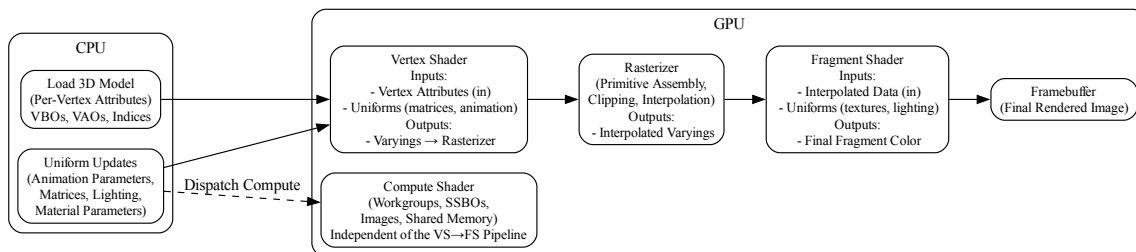
Fig. 5.19: Shaders input and output
