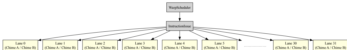
Fig. 6.14: In dual-issue mode , Chime A carries floating-point data while Chime B carries integer data—both issued by the same CUDA thread. In contrast, under time-sliced execution , Chime A and Chime B carry either floating-point or integer data independently, and are assigned to separate CUDA threads.
