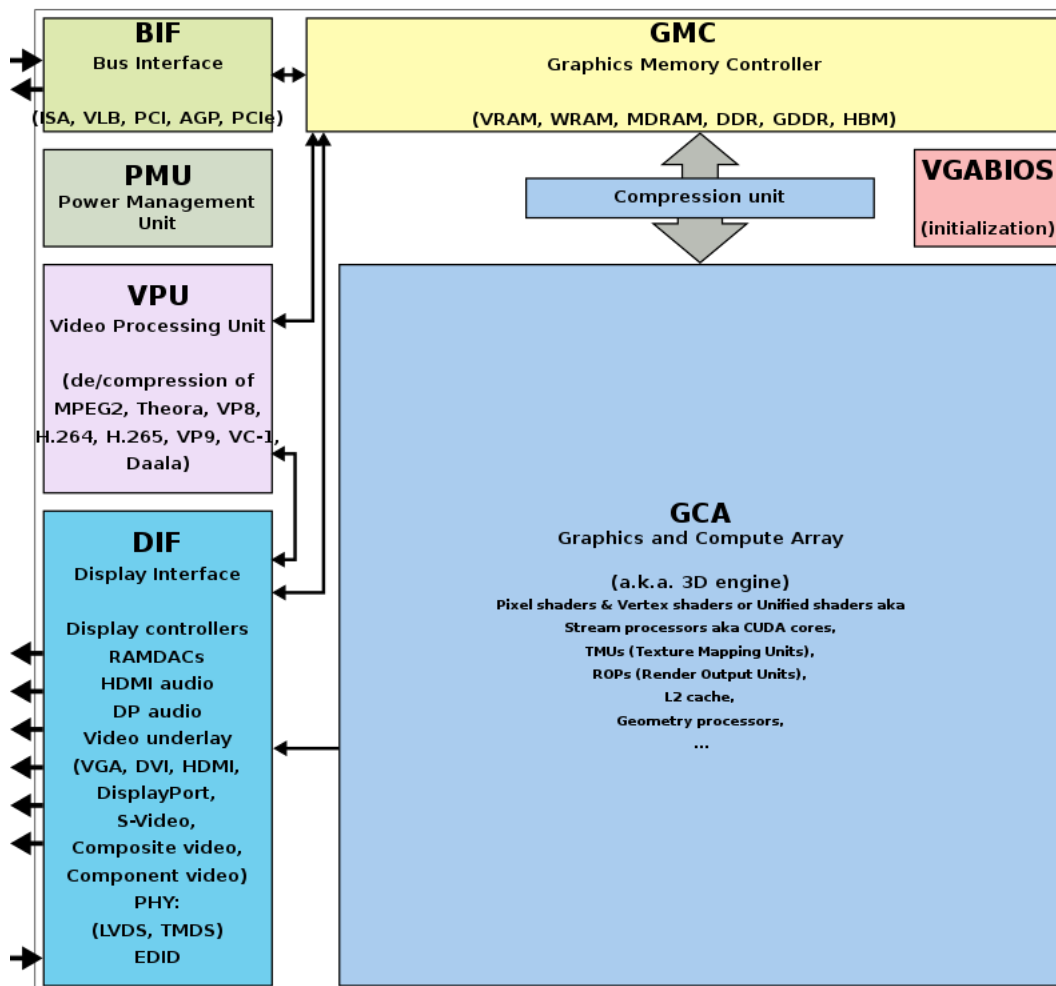
Fig. 6.2: Components of a GPU: GPU has accelerated video decoding and encoding Page 107, 2
