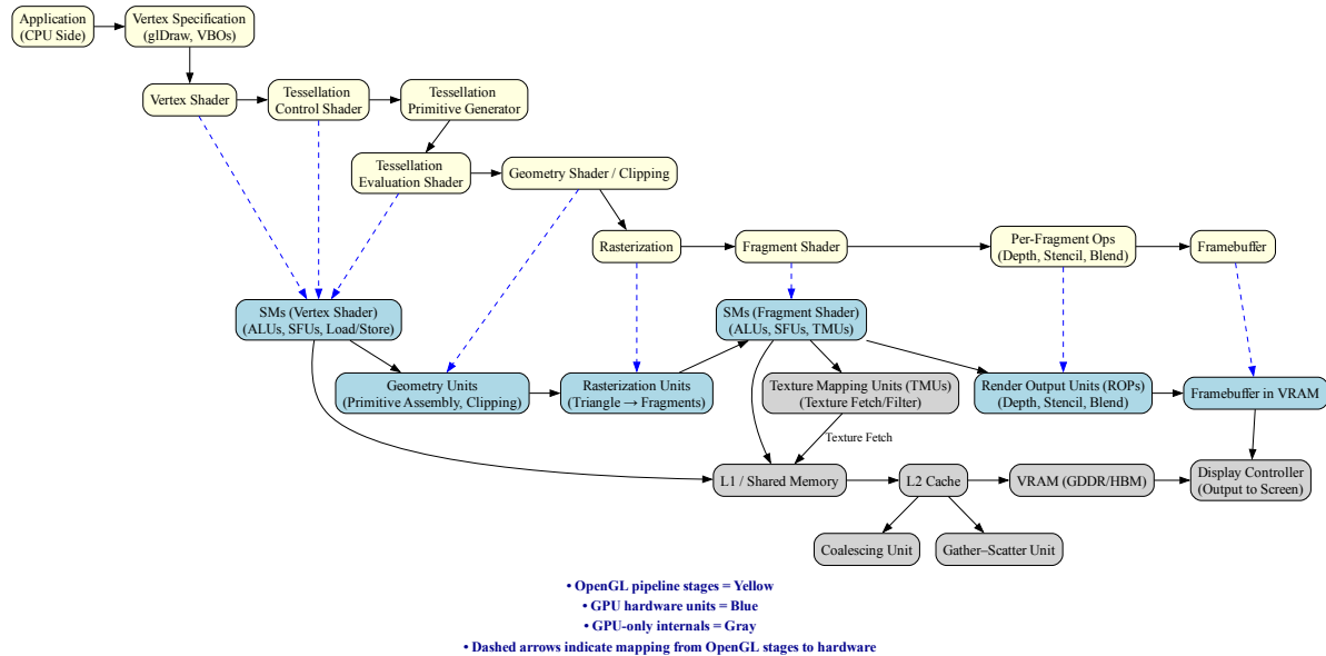
Fig. 6.22: The stages of OpenGL pipeline and GPU's acceleration components
