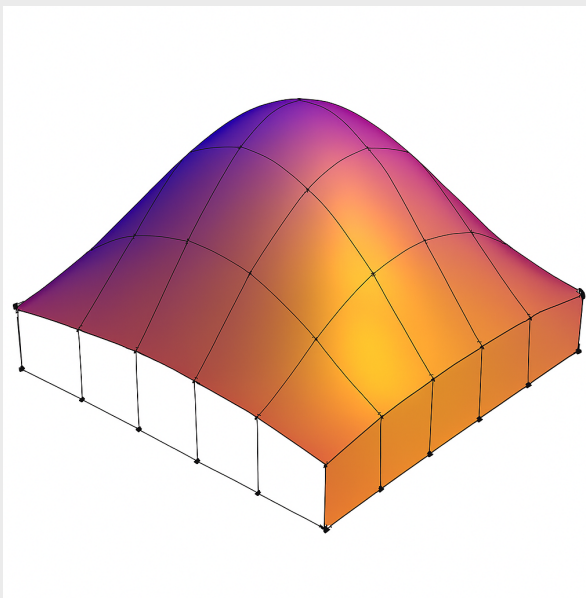
Fig. 5.8: The final rendering result for 5x5 tessellated mesh.
