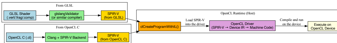
Fig. 7.4: Compiling and Deploying GPU Code from GLSL, Vulkan, and OpenCL
