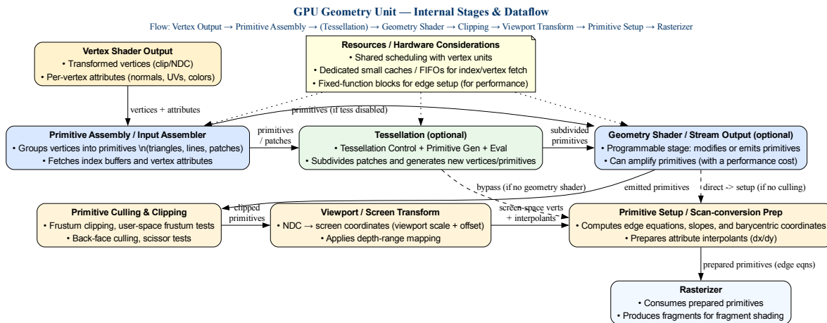
Fig. 6.26: Geometry Unit with its sub-functions (assembly, tessellation, clipping, viewport transform, etc.)
