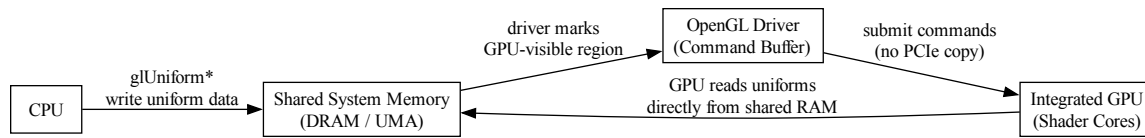
Fig. 6.19: CPU send Uniform Updates Data to iGPU for rendering
