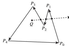
Fig. 4.12: Draw a polygon with vertices counter clockwise
