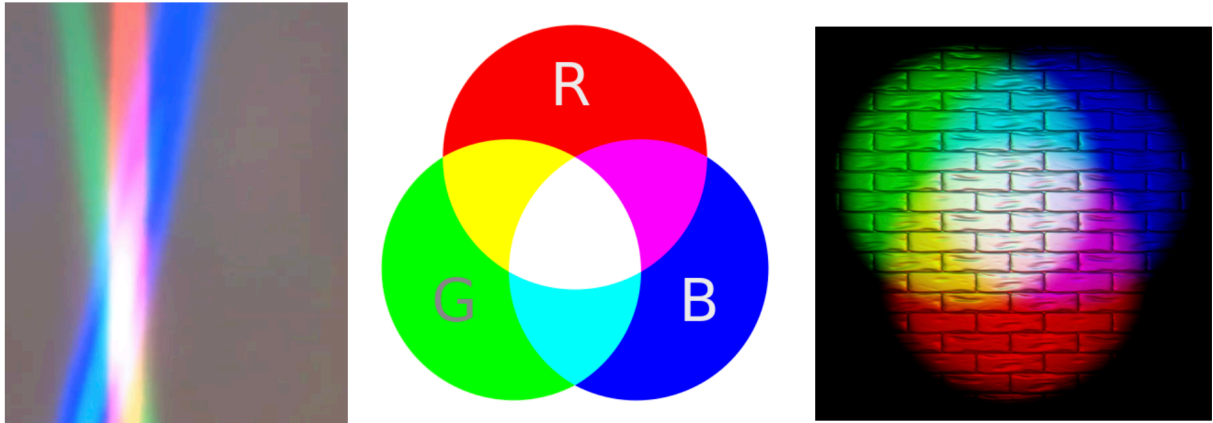
Fig. 4.1: Additive colors in light
