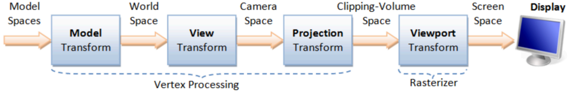
Fig. 4.2: Coordinate Transformation Pipeline Page 32, 4
