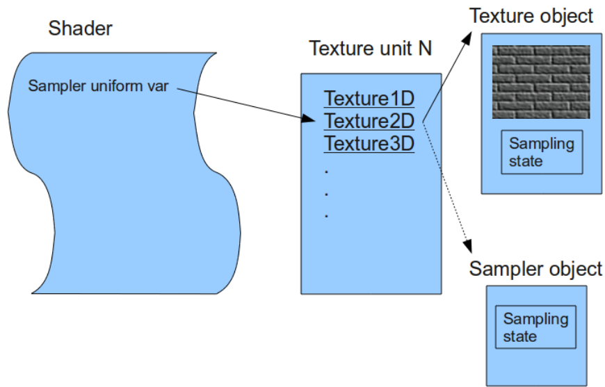
Fig. 5.20: Relationships between the texturing concept Page 101, 35 .
