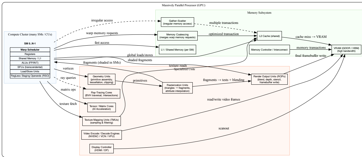
Fig. 6.3: Components of a GPU: SIMD/SIMT + several specialized processing units
