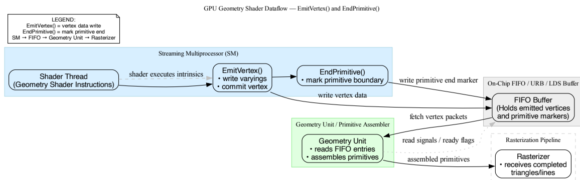
Fig. 6.25: Micro-level flow: SM → Geometry Unit via Emit/Cut
