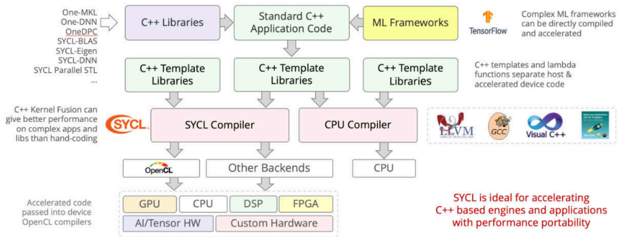
Fig. 7.12: SYCL = C++ template and compiler for Data Parallel Applications on AI on CPUs, GPUs and HPGAs.
