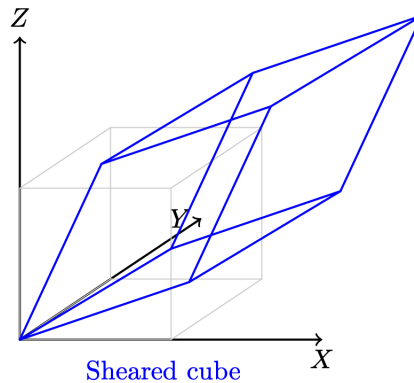
Fig. 4.3: 3D shear
