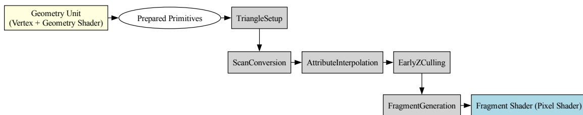
Fig. 6.27: Rasterization pipeline
