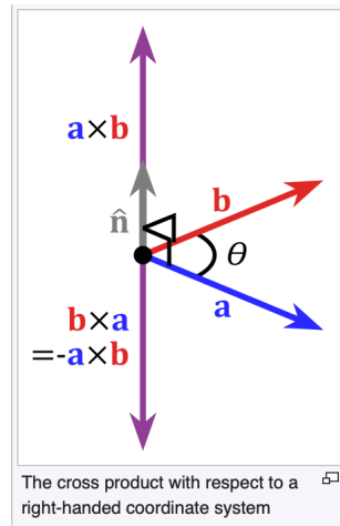
Fig. 4.13: Cross product definition in 3D
