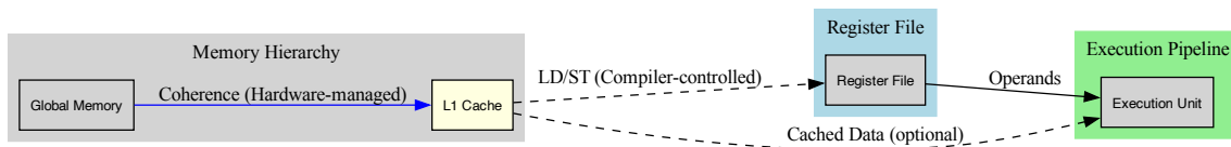
Fig. 6.20: Operand Delivery in Traditional GPU (Traditional Model: Register File + L1 Cache)
