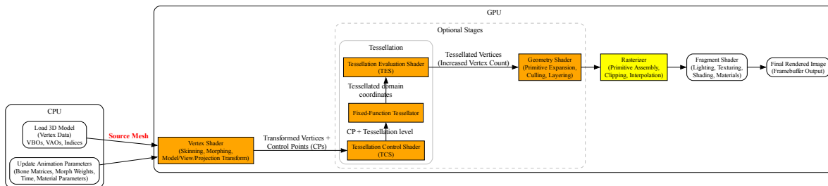
Fig. 5.15: CPU and GPU Traditional Pipeline For Shaders
