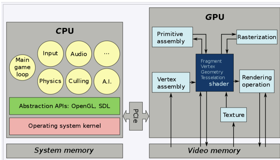
Fig. 3.1: Components of a GPU: GPU has accelerated video decoding and encoding Page 21, 1
