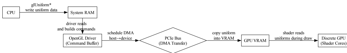
Fig. 6.18: CPU send Uniform Updates Data to dGPU for rendering
