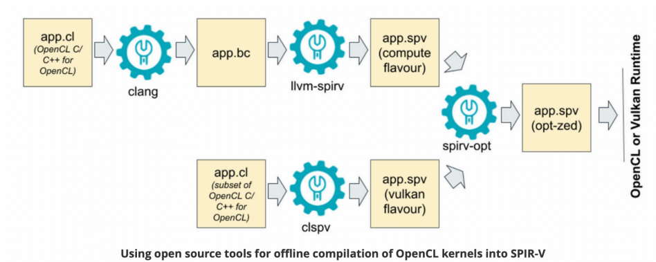
Fig. 7.2: Offline Compilation of OpenCL Kernels into SPIR-V Using Open Source Tooling Page 157, 11
