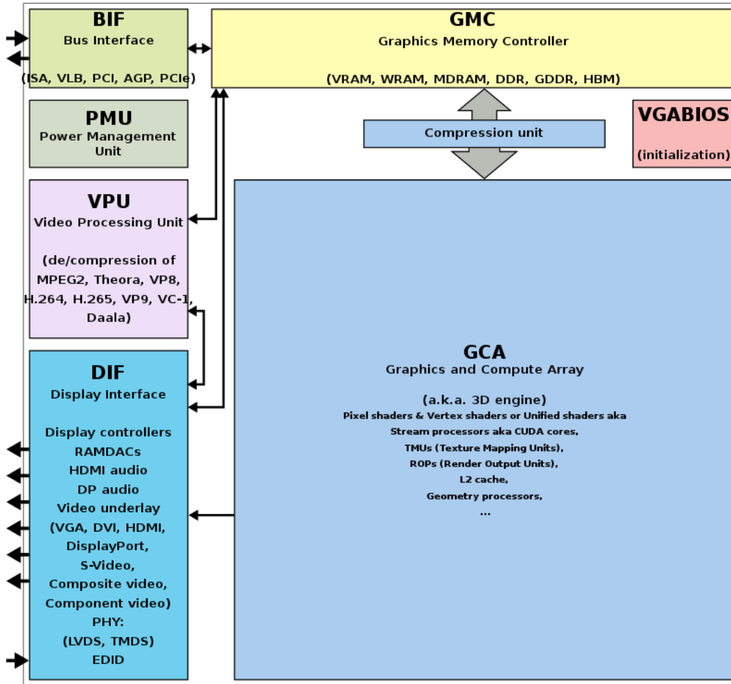
Fig. 3.1: Components of a GPU: GPU has accelerated video decoding and encoding Page 21, 1
