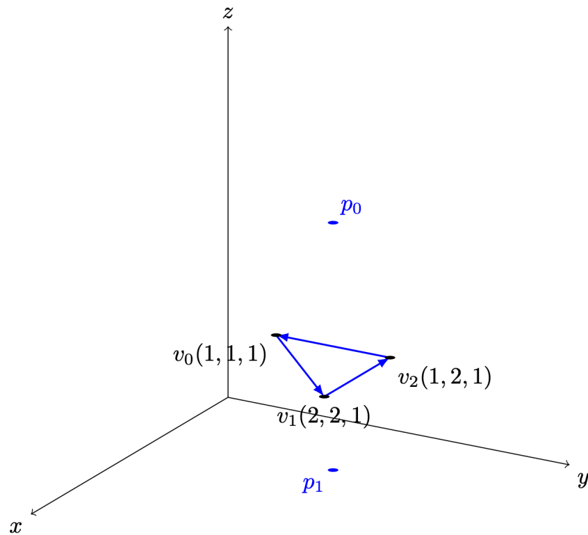
Fig. 4.17: A triangle can be constructed as soon as three vertices are received
