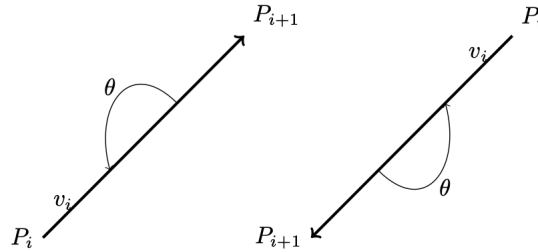
Fig. 4.8: Inward and outward in 2D for a vector.
