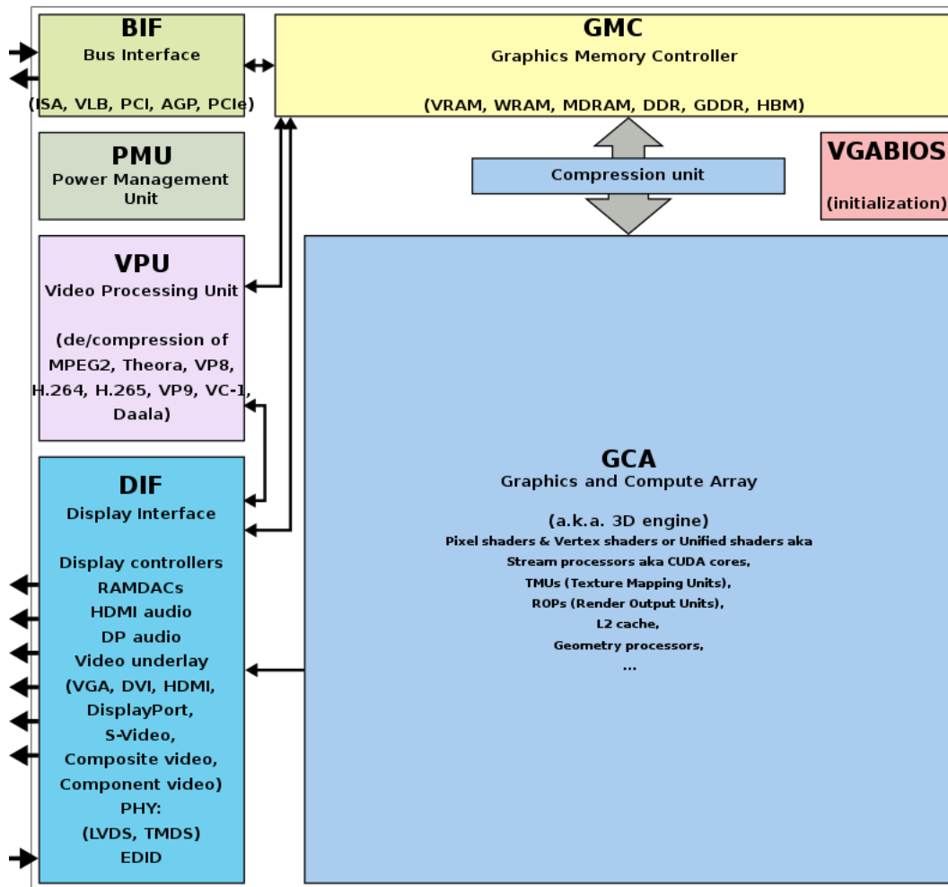
Fig. 3.5: Components of a GPU: GPU has accelerated video decoding and encoding 10
