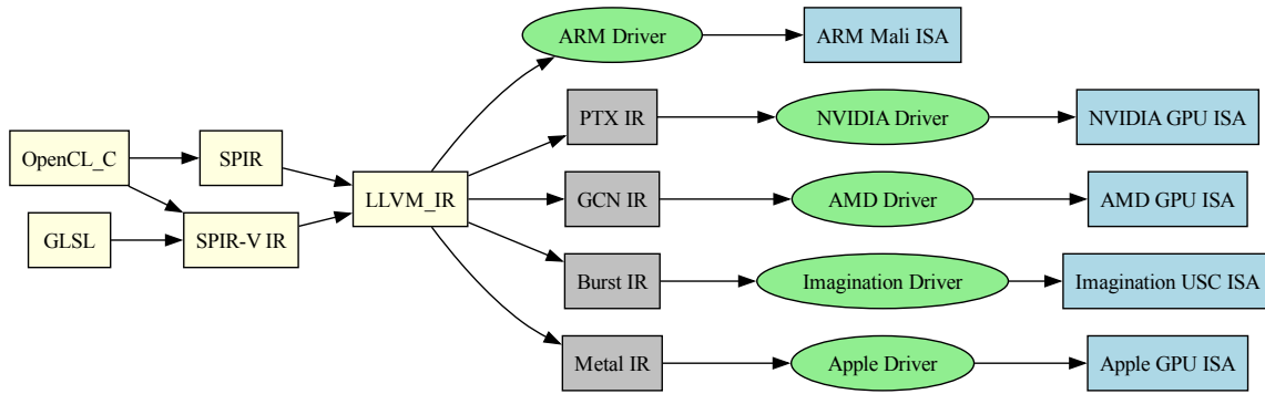
Fig. 6.6: Graphics and OpenCL Compiler IR Conversion Flow
