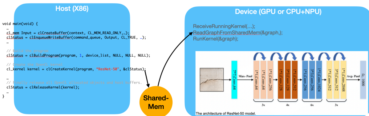
Fig. 6.11: Implement ML graph scheduler both on compiler and runtime
