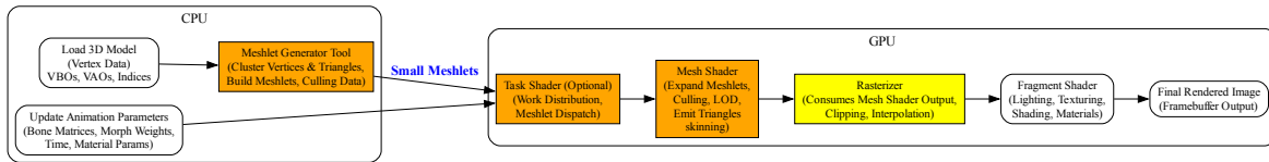
Fig. 4.17: CPU and GPU Mesh Shader Pipeline For Shaders
