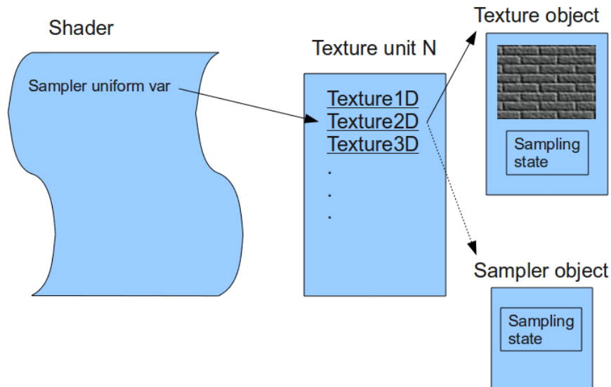
Fig. 4.19: Relationships between the texturing concept 34 .
