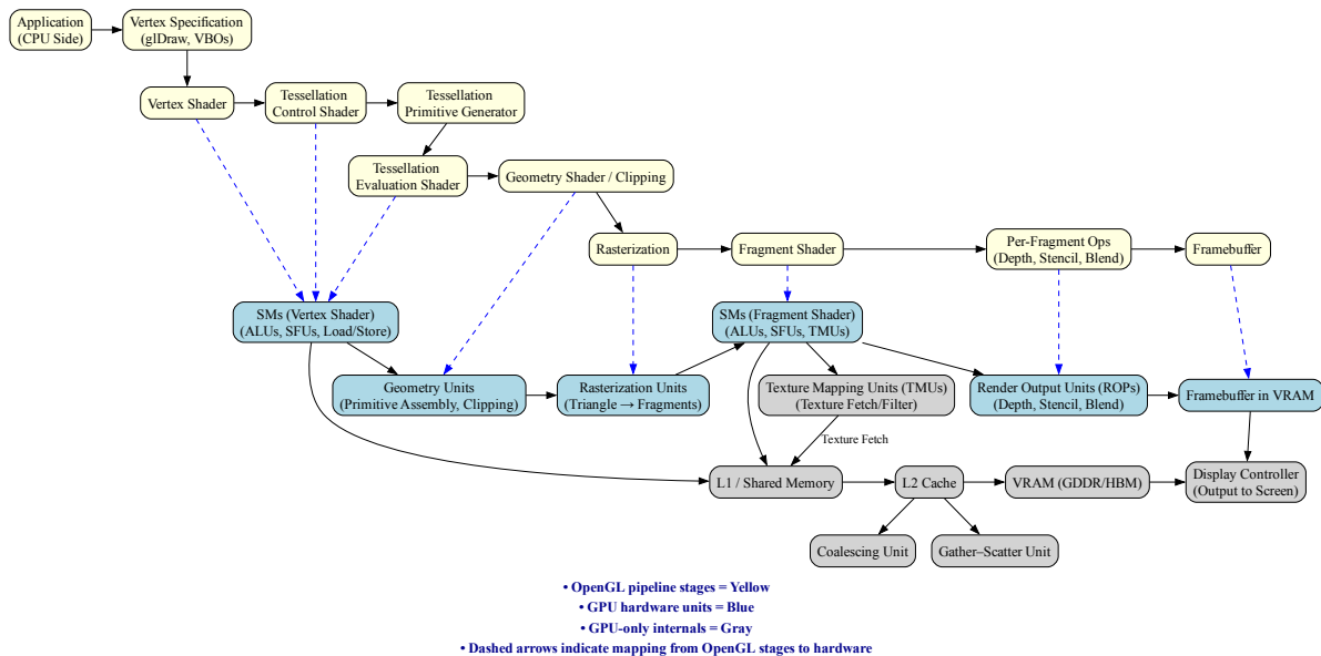
Fig. 5.4: The stages of OpenGL pipeline and GPU's acceleration components
