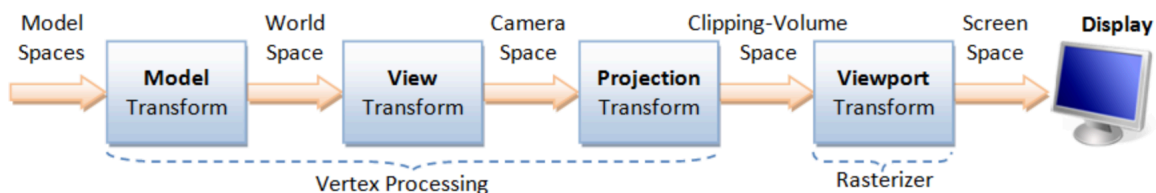
Fig. 3.15: Coordinates Transform Pipeline Page 29, 1
