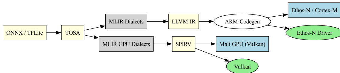
Fig. 6.9: ARM IR Conversion Flow
