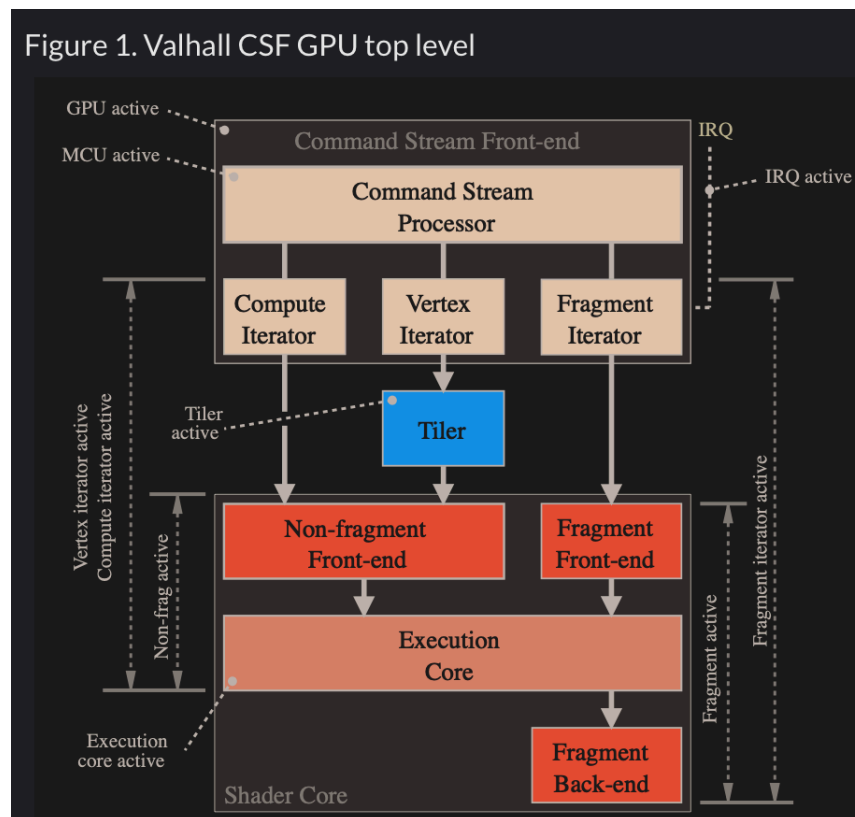
Fig. 3.7: MCU and specific HW circuits to speedup the processing of CSF (Command Stream Fronted) Page 22, 14 .
