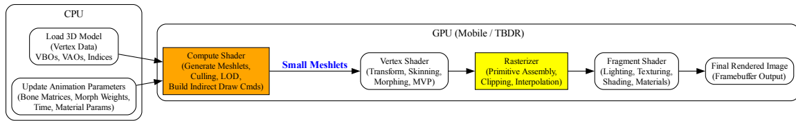
Fig. 4.16: CPU and GPU Mobile Pipeline For Shaders
