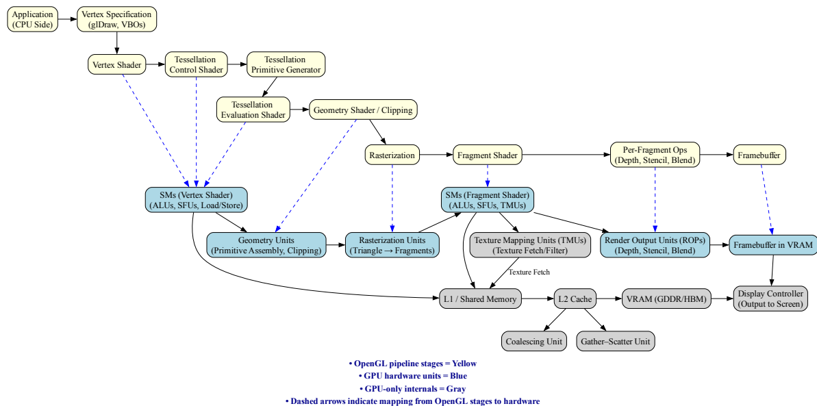
Fig. 5.20: The stages of OpenGL pipeline and GPU's acceleration components
