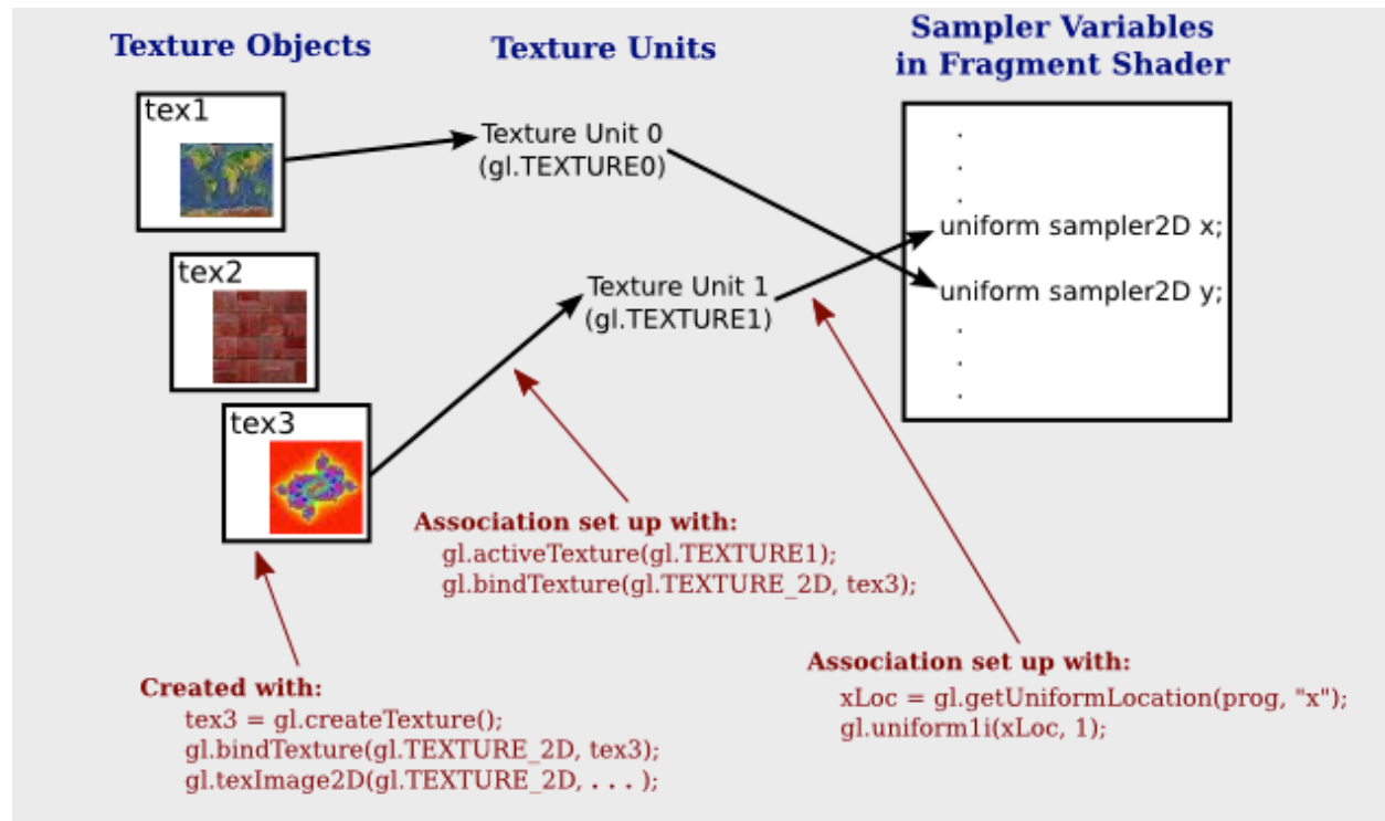
Fig. 4.20: Binding sampler variables 35 .
