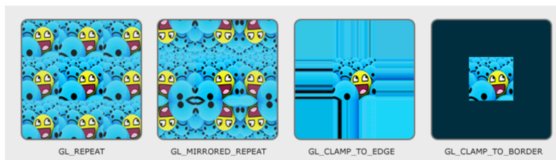
Fig. 5.28: Texture Warpping 27
