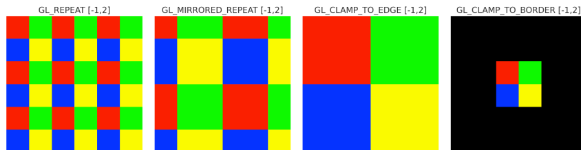
Fig. 5.27: Texture Warpping
