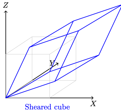
Fig. 3.16: 3D shear
