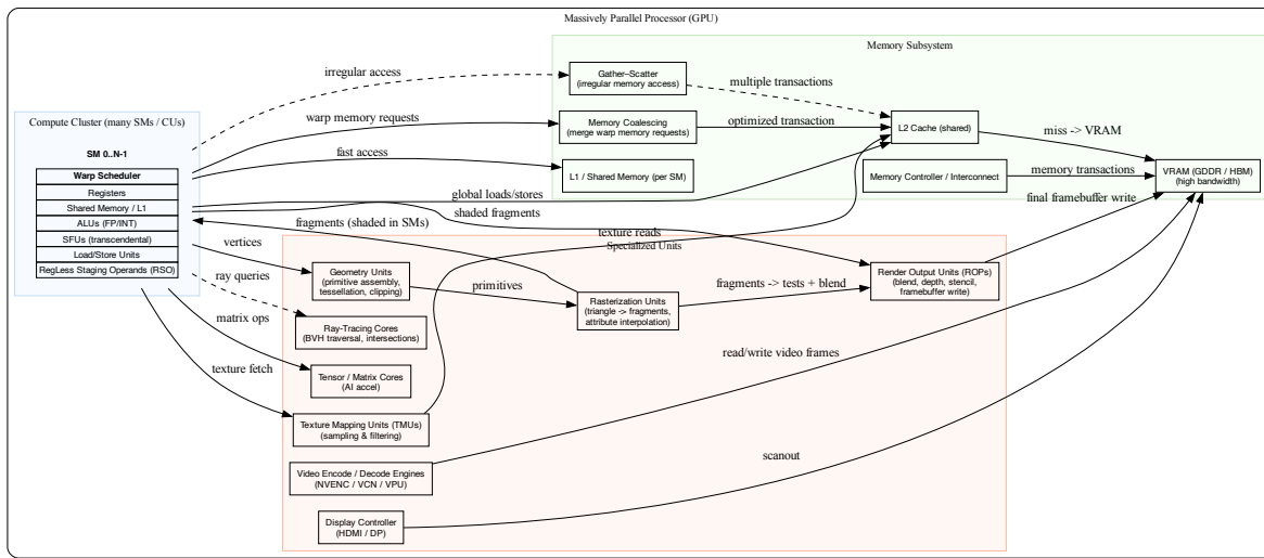
Fig. 5.3: Components of a GPU: SIMD/SIMT + several specialized processing units
