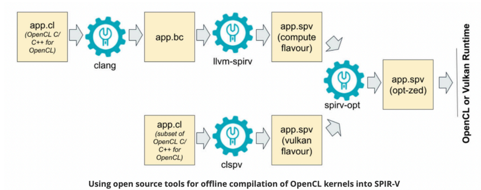
Fig. 6.2: Offline Compilation of OpenCL Kernels into SPIR-V Using Open Source Tooling Page 143, 10
