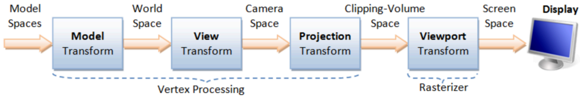
Fig. 3.32: Coordinates Transform Pipeline Page 29, 1
