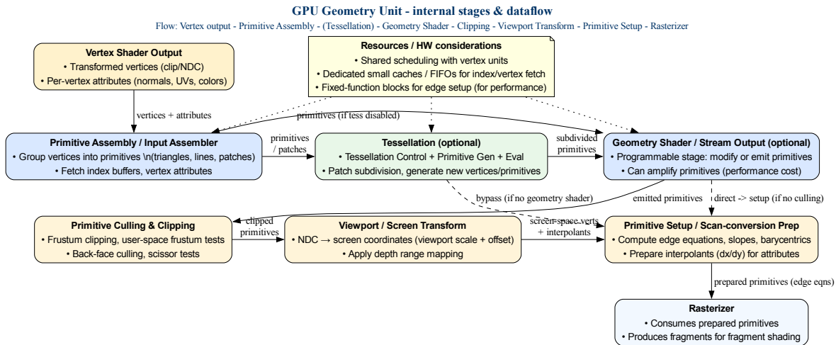
Fig. 5.24: Geometry Unit with its sub-functions (assembly, tessellation, clipping, viewport transform, etc.)
