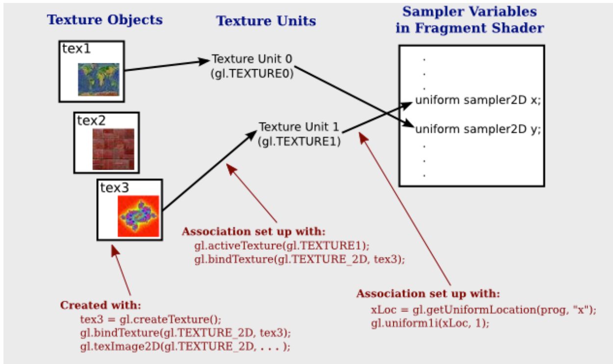
Fig. 5.24: Binding sampler variables Page 109, 43 .
