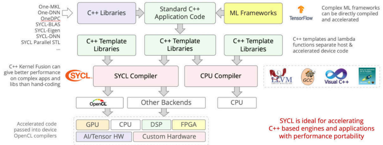
Fig. 7.13: SYCL = C++ template and compiler for Data Parallel Applications on AI on CPUs, GPUs and HPGAs.
