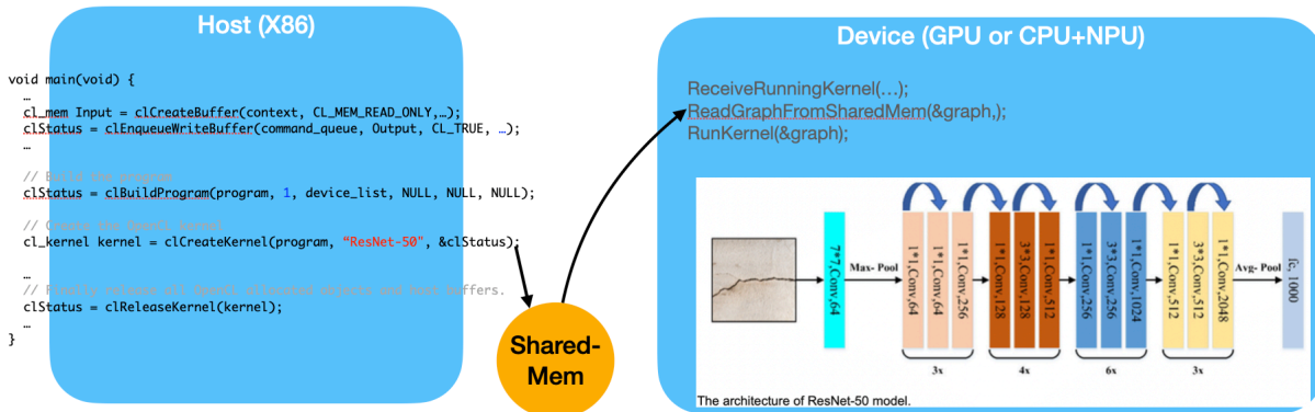
Fig. 7.12: ML graph scheduling in both the compiler and runtime
