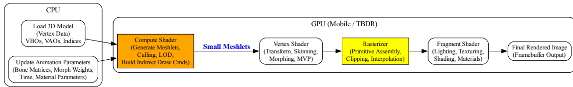
Fig. 5.19: CPU and GPU Mobile Pipeline For Shaders
