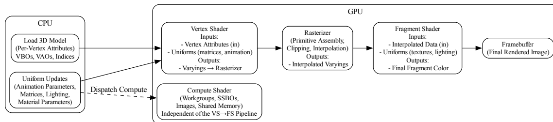
Fig. 5.22: Shaders input and output
