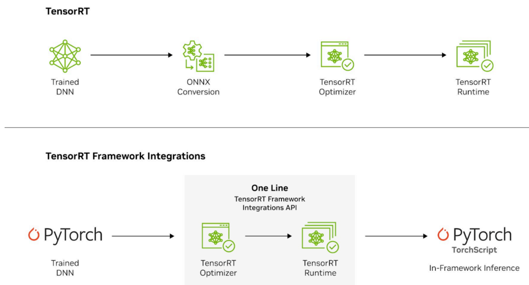
Fig. 7.8: Tensor-RT
