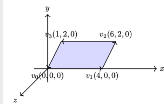
Fig. 4.6: The area and plane face determined by v_0, v_1, v_2 with CCW ordering after rotation z axis.
