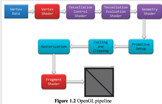
Fig. 5.6: OpenGL pipeline in blue book
