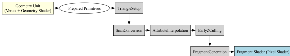
Fig. 6.27: Rasterization pipeline
