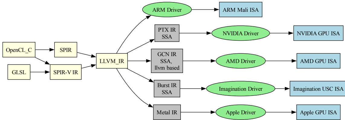
Fig. 7.6: Graphics and OpenCL Compiler IR Conversion Flow
