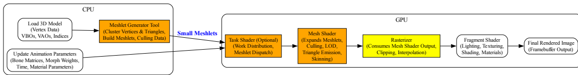
Fig. 5.20: CPU and GPU Mesh Shader Pipeline For Shaders
