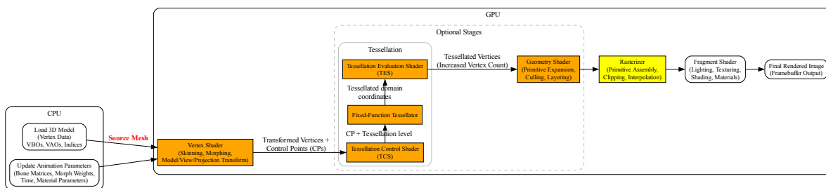
Fig. 5.18: CPU and GPU Traditional Pipeline For Shaders
