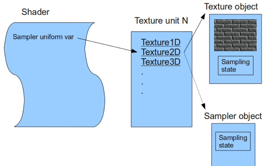
Fig. 5.23: Relationships between the texturing concept 42 .
