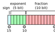
Fig. 5.2: IEEE 754 half precision of Floating point representation 2
