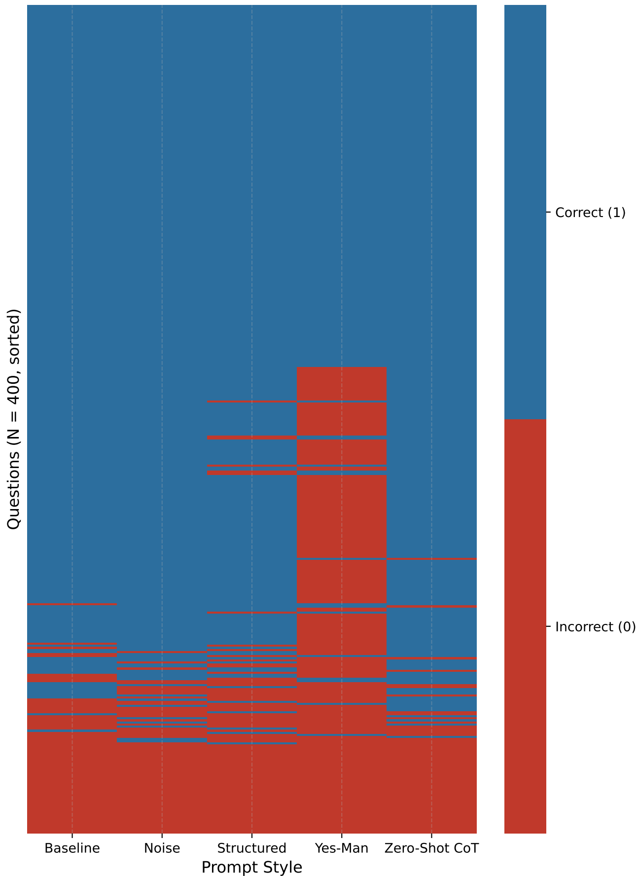
Evaluation Matrix — Correctness by Question and Prompt Style (sorted by total correct answers, highest at top)
