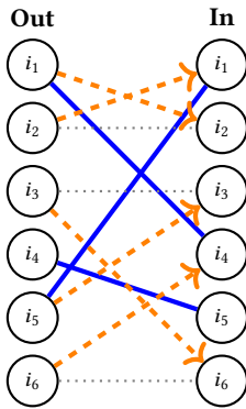
(b) JBC + augmenting path
