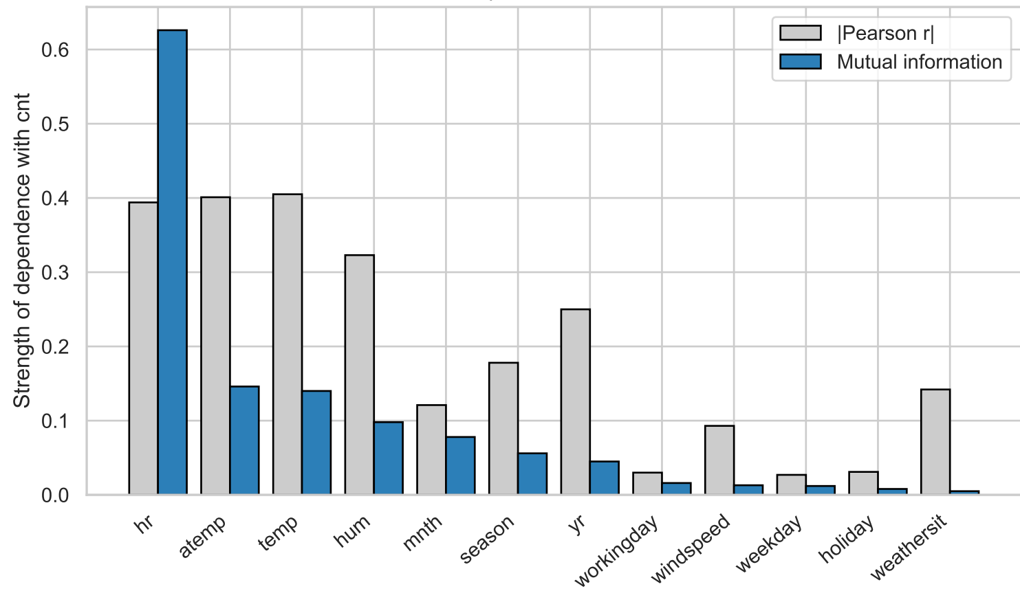
Non-linear dependence: MI vs Pearson r
