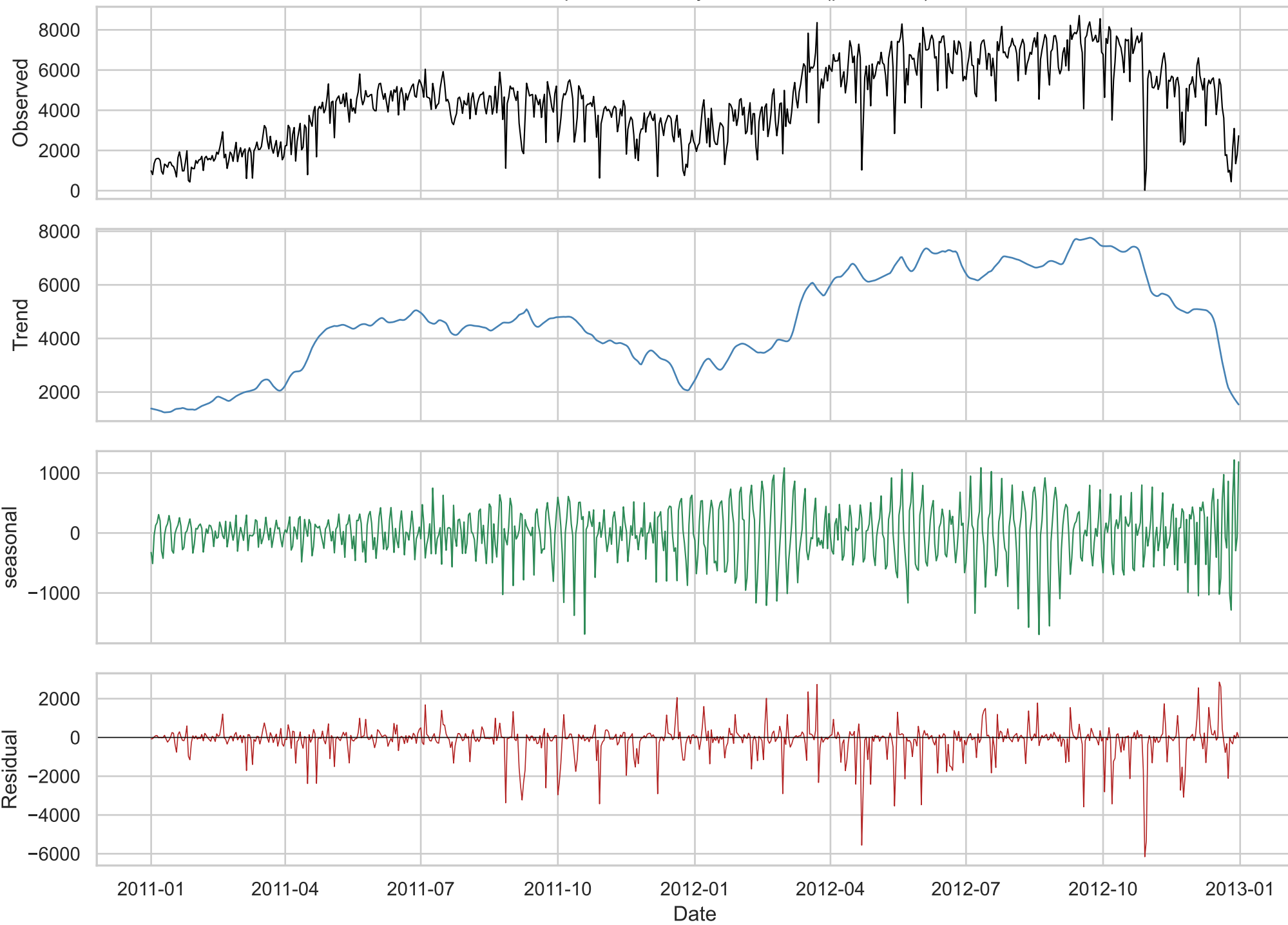
STL decomposition of daily total rentals (period = 7)
