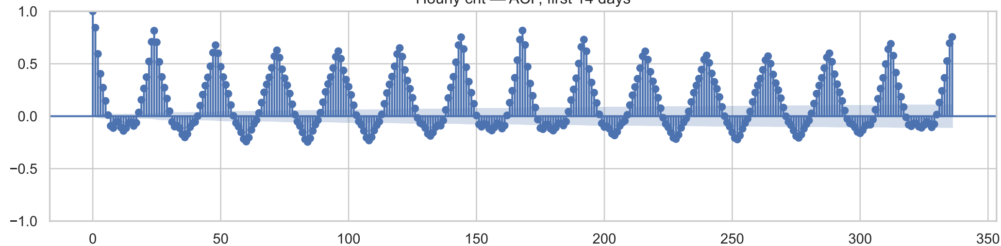
Hourly cnt — ACF, first 14 days
