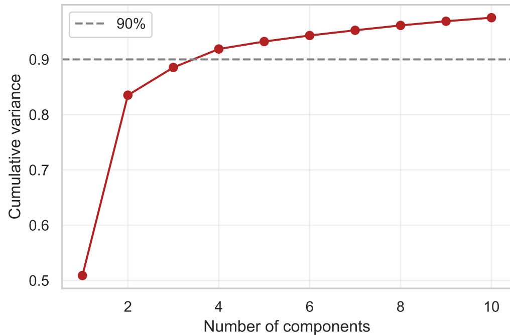
Cumulative variance
