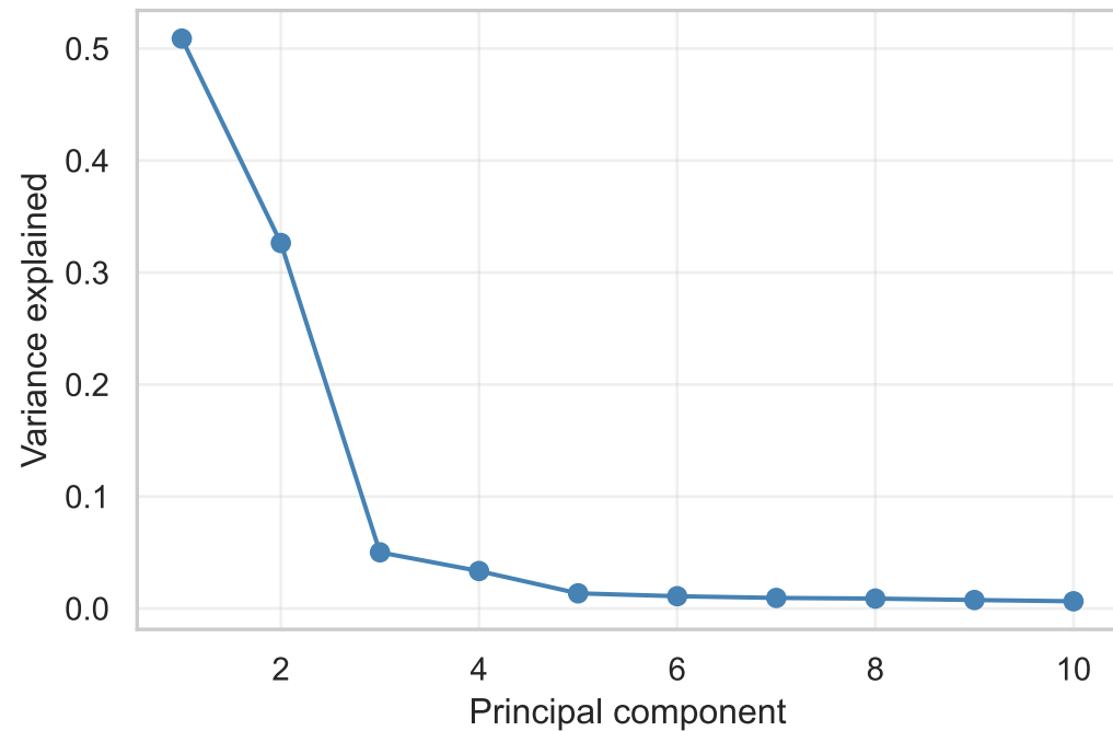
Scree plot
