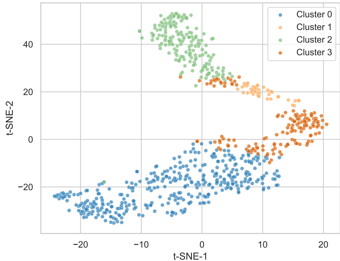
t-SNE embedding, colored by K-means cluster
