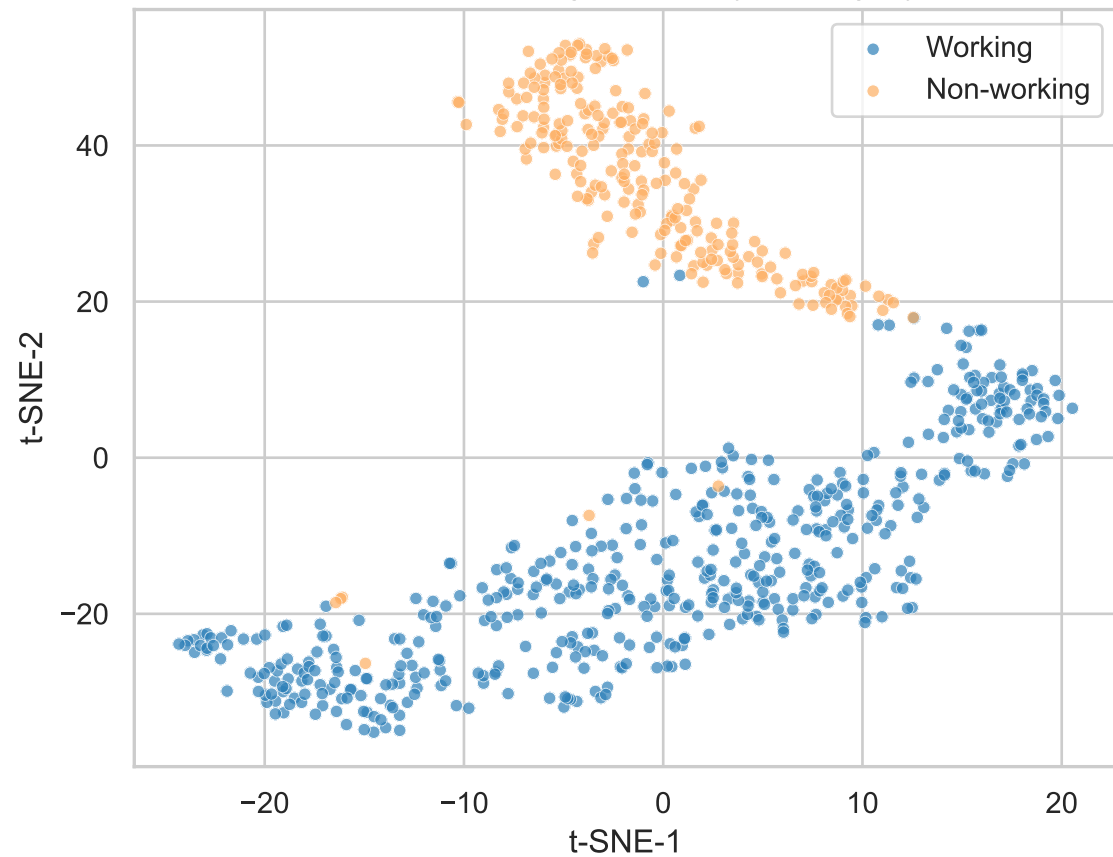
t-SNE embedding, colored by workingday
