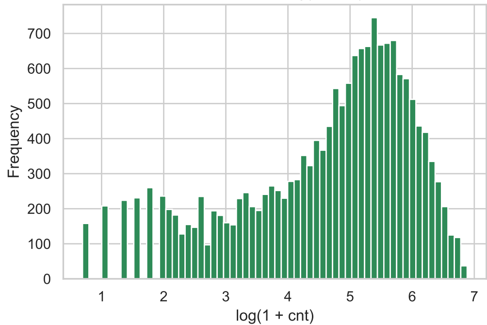
Distribution of \log(1 + \text{cnt})
