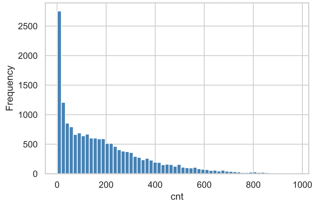
Distribution of hourly cnt (raw)
