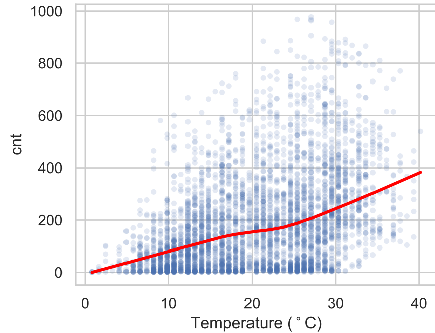
cnt vs temperature
