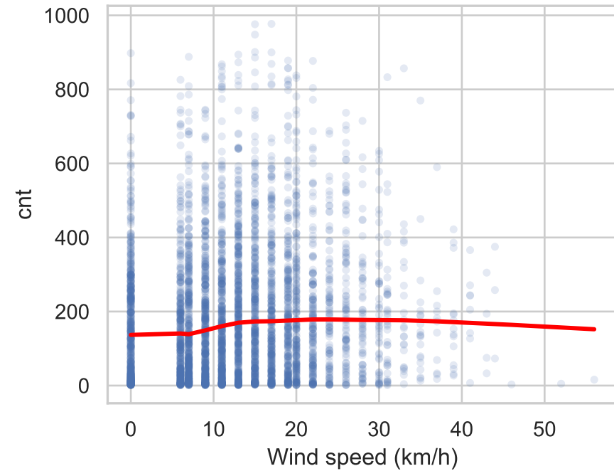
cnt vs wind speed
