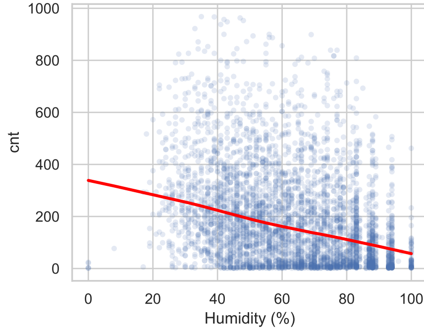
cnt vs humidity
