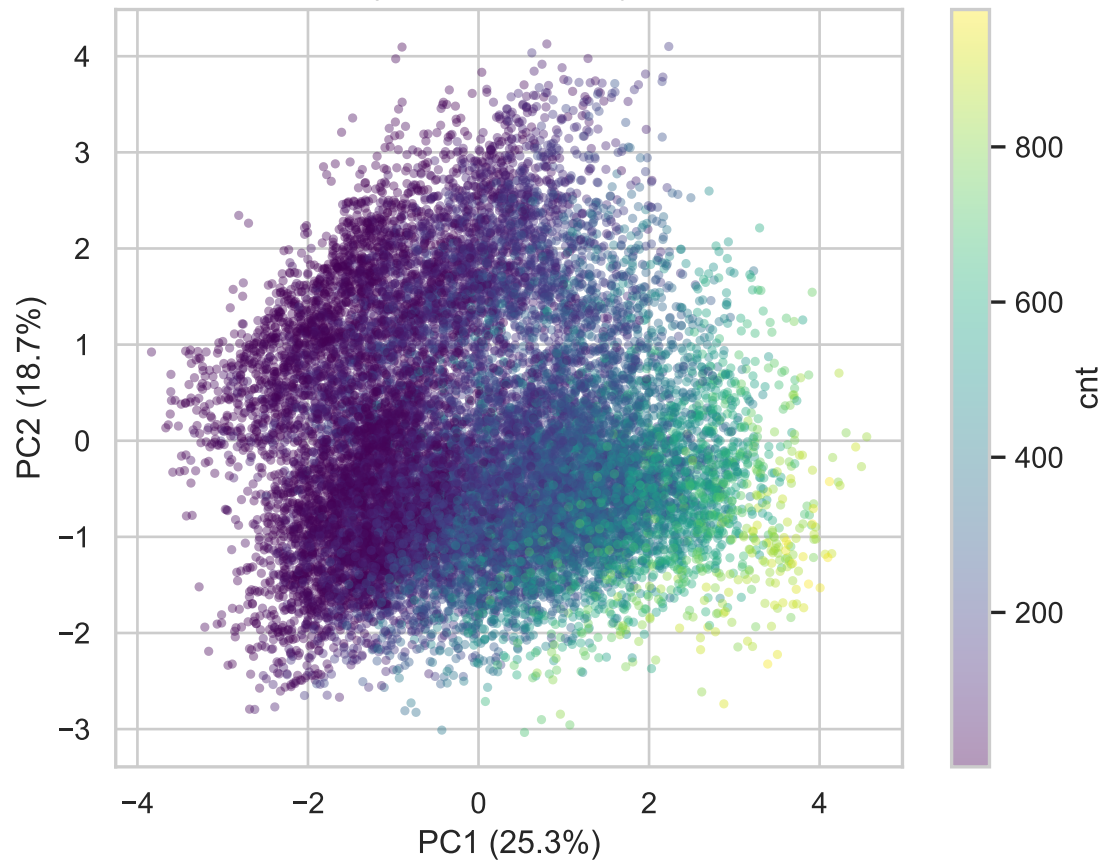
Same projection, colored by actual cnt
