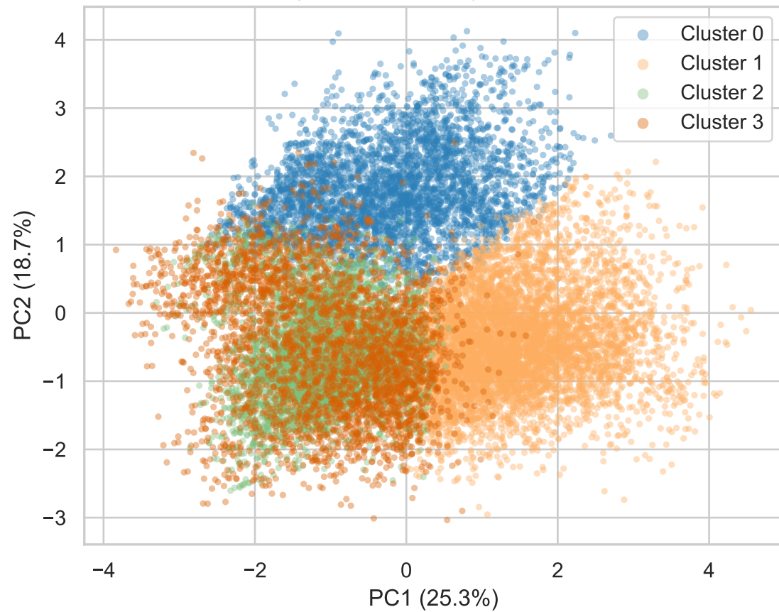
PCA projection, colored by K-means cluster
