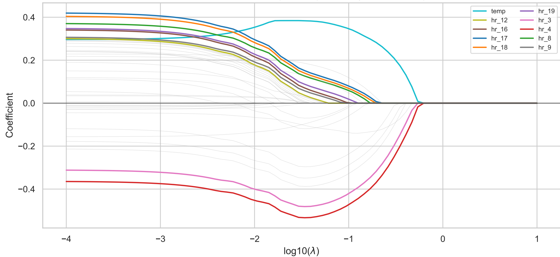
Lasso coefficient paths (top-10 by final magnitude colored)
