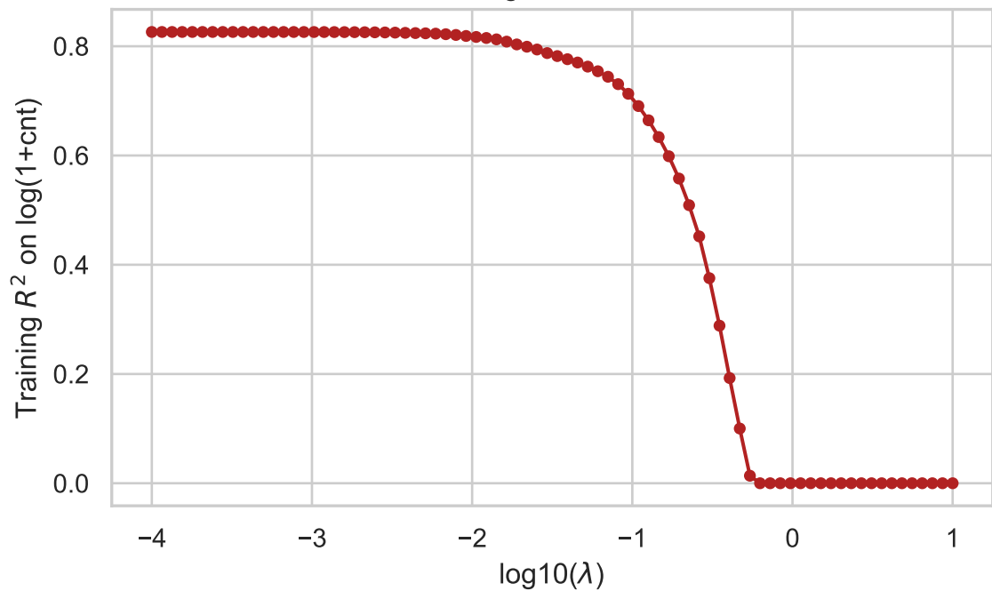
Training fit vs lambda
