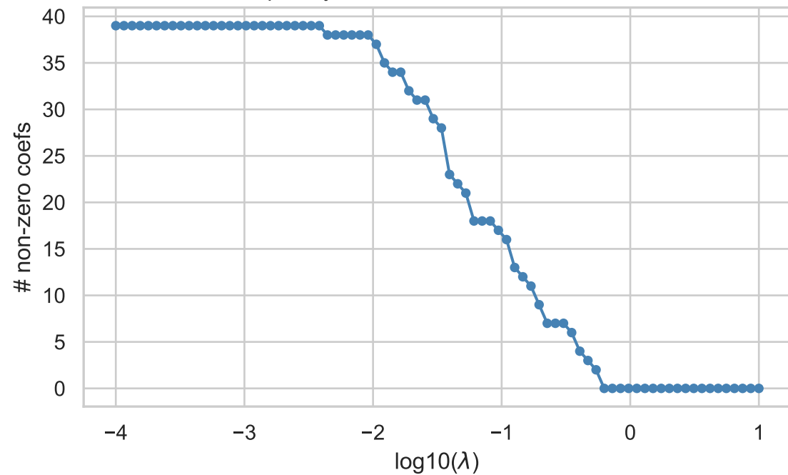
Sparsity of Lasso solution vs lambda
