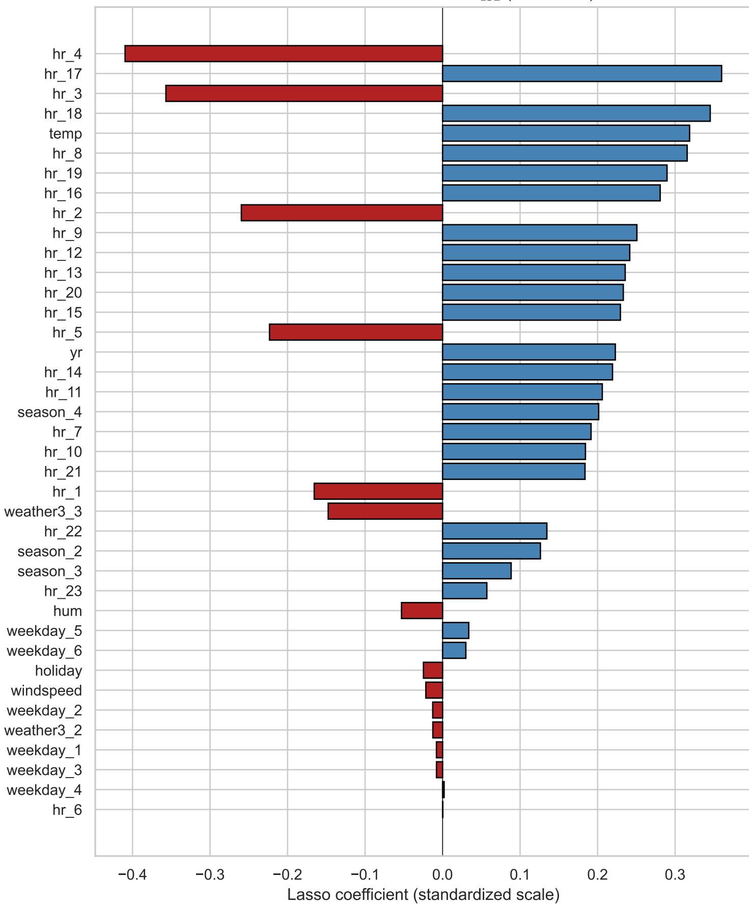
Lasso-selected coefficients at \lambda_{1SE} (n=39 of 40)
