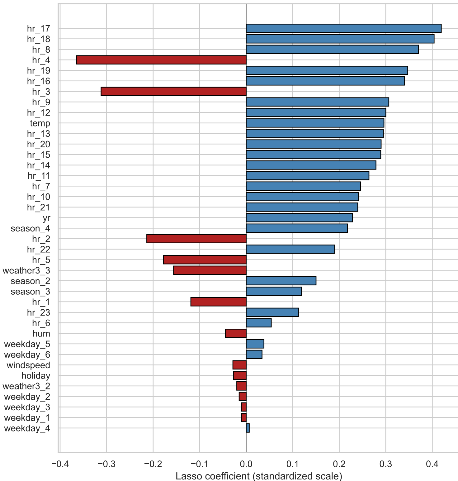
Coefficients at \lambda_{\min} (n=39 of 40; effectively OLS)
