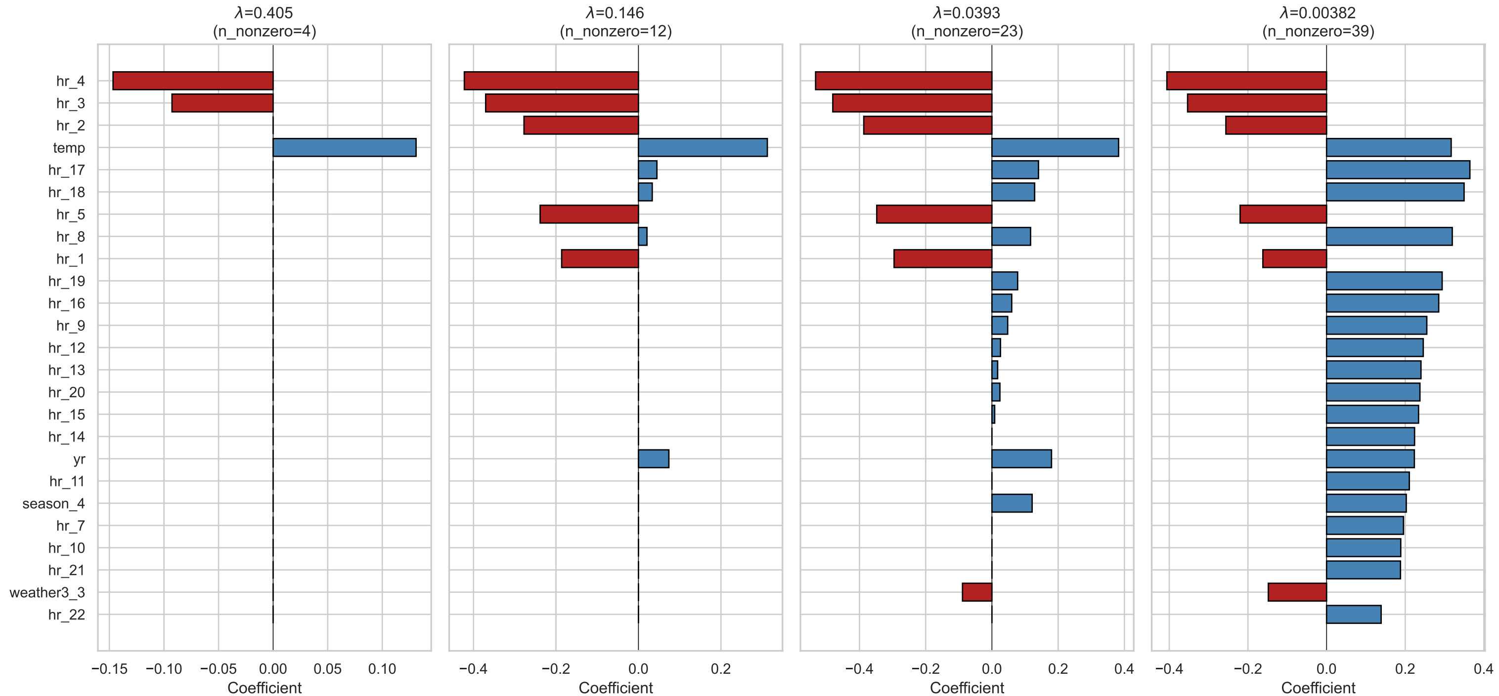
Top-25 coefficients at four lambdavalues (top: largest magnitude)
