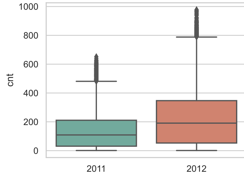
cnt by year
