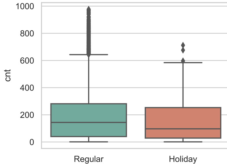
cnt: regular day vs holiday
