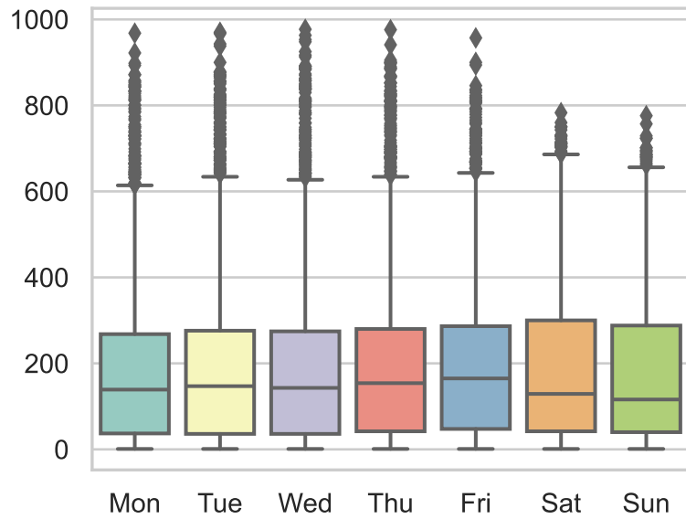
cnt by weekday
