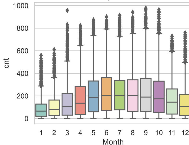
cnt by month
