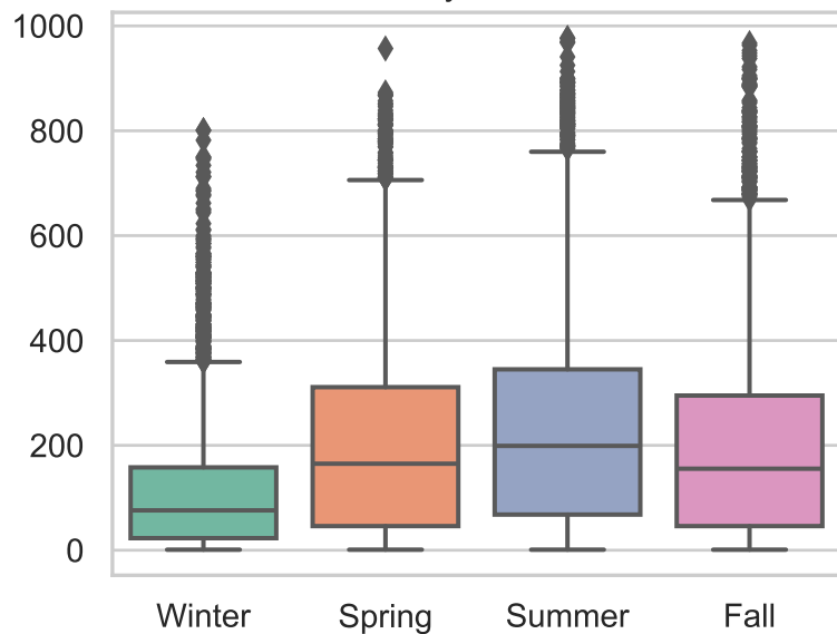
cnt by season
