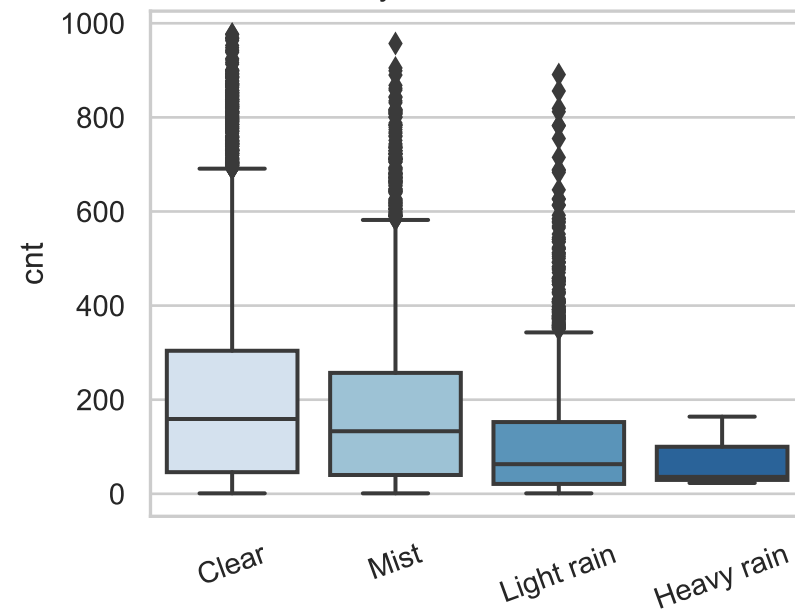
cnt by weather situation
