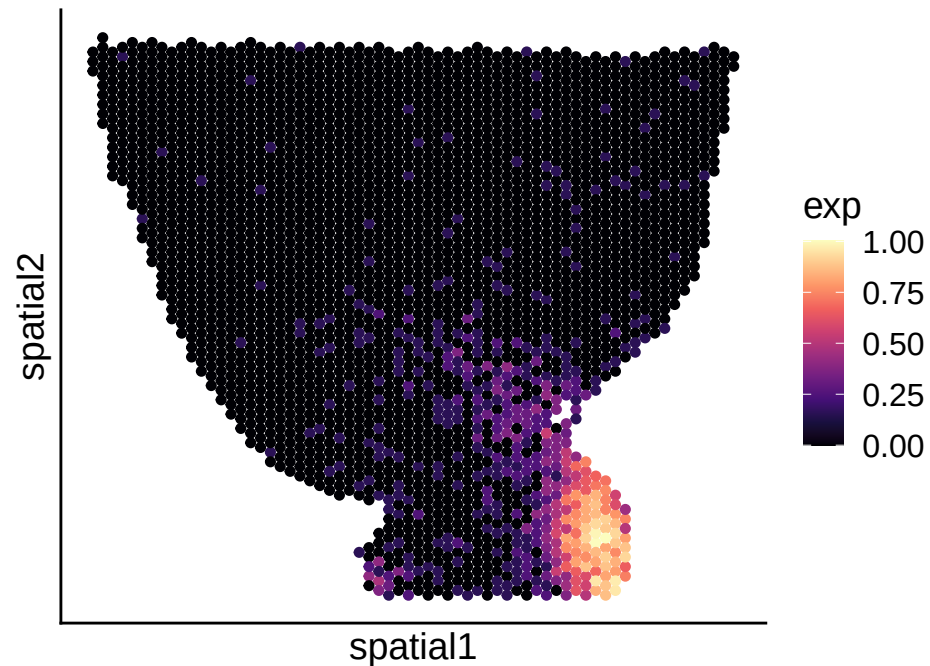
S100a5: simulated data 10% signal
